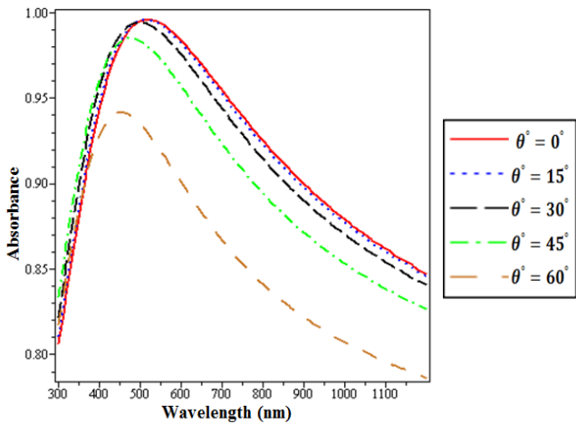
Fig. 5 Average of absorbance versus the wavelength for different angles of incidence with \epsilon_1 = 3.24 , L_1 = 70 \text{ nm} , L_2 = 3.97 \mu\text{m} and \epsilon_2 = -7.993275 + i0.7050 .
