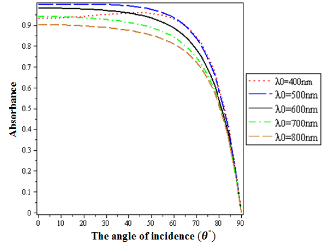
Fig. 8 Average of absorption versus the angles of incidence for different wavelengths with \epsilon_1 = 3.24 , L_1 = 70 \text{ nm} , L_2 = 3.97 \mu\text{m} and \epsilon_2 = -10.720504 + i0.884790 .
