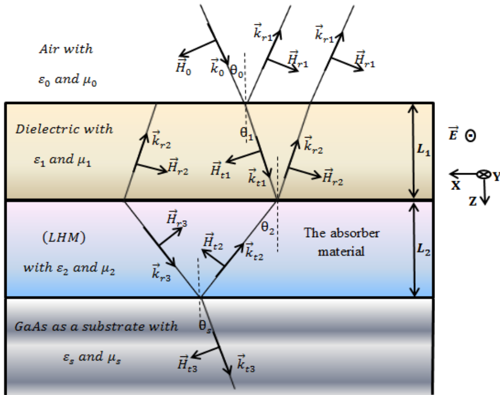
Fig. 1 Schematic diagram of the investigated DLARC structure under TE polarization of light.
