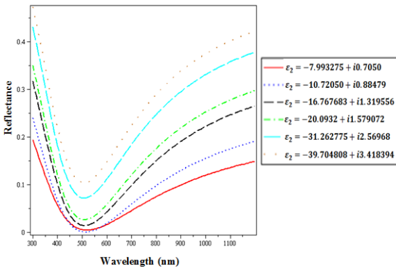
Fig.2 Average of reflectance versus the wavelength for different \epsilon_2 for the LHM with \epsilon_1=3.24 , L_1=70 nm and L_2=3.97 \mu\text{m} under normal incidence.
