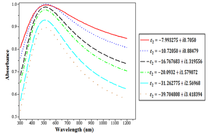
Fig.4 Average of absorbance versus the wavelength for different \epsilon_2 for the LHM with \epsilon_1=3.24 , L_1=70 nm and L_2=3.97 \mu\text{m} under normal incidence.
