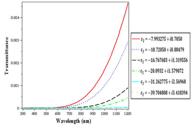
Fig.3 Average of transmittance versus the wavelength for different \epsilon_2 for the LHM with \epsilon_1=3.24 , L_1=70 nm and L_2=3.97 \mu\text{m} under normal incidence.
