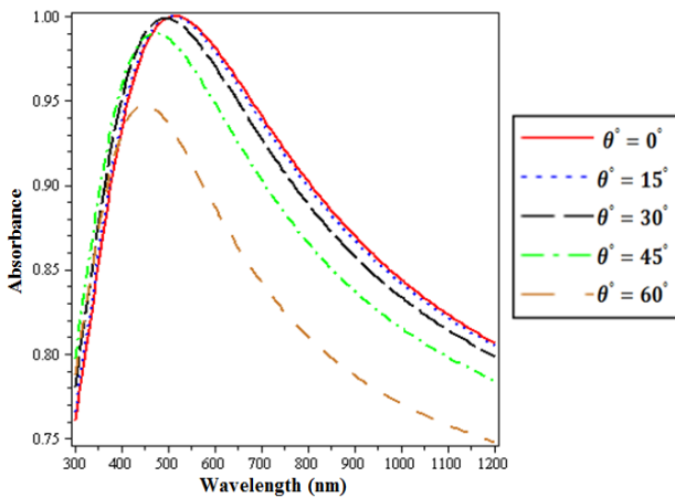
Fig.6: Average of absorbance versus the wavelength for different angles of incidence with \epsilon_1 = 3.24 , L_1 = 70 \text{ nm} , L_2 = 3.97 \mu\text{m} and \epsilon_2 = -10.720504 + i0.884790 .
