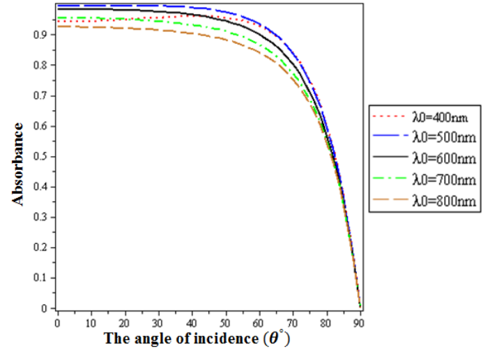
Fig. 7: Average of absorbance versus the angles of incidence for different wavelengths with \epsilon_1 = 3.24 , L_1 = 70 \text{ nm} , L_2 = 3.97 \mu\text{m} and \epsilon_2 = -7.993275 + i0.7050 .
