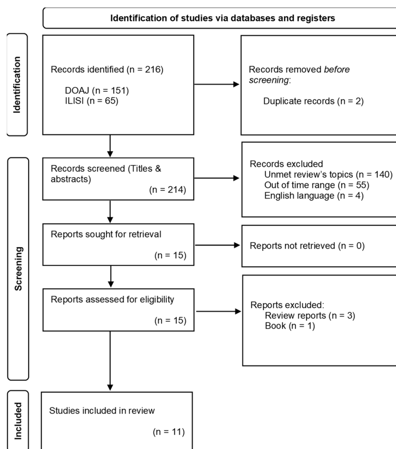
Figure 1. PRISMA flow diagram adapted from [34]. For more information, visit: http://www.prisma-statement.org/ (accessed on 15 March 2023).
