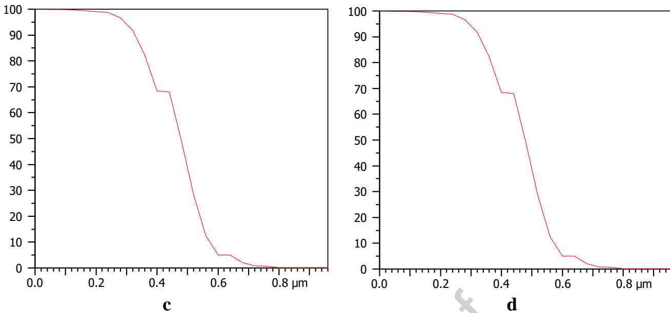
Fig. 7 (a) Furrows particle parameters showing the Maximum depth of furrows of 0.5527\mu\text{m} , Mean depth of 0.1342\mu\text{m} and Mean density of 4.582\text{ cm/cm}^2 (b) the furrows deeper than the threshold are showing Parameters of Maximum depth of furrows 0.5527\mu\text{m} at Mean depth of 0.3565\mu\text{m} Mean density of 0.07749\text{cm/cm}^2 (c) Curve display mode Particle count distribution log curve (d) Area curve
