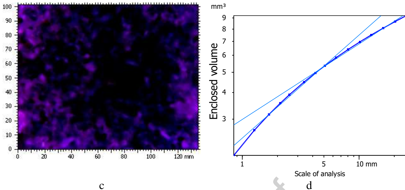
Fig. 5 (a) Step height calculations of z-difference of 0.1464\mu\text{m} (b) SEM intensity surface image (c) Cell pattern on the scaffold Filled point of KL transformed (d) Morphological envelopes Fractal analysis of dimension 2.64
