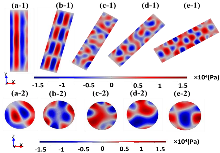
Fig. 2. Acoustic pressure field in the circular glass capillary with different tilting angle (a) parallel, (b) 15°, (c) 30°, (d) 45°, (e) 60°. (1) is the top view and (2) is the cross-sectional view.
