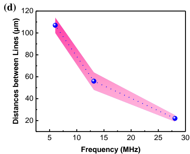
Fig. 7. The patterning in the circular glass capillary with different frequencies: (a) 6.05 MHz, (b) 13.15 MHz, and (c) 27.37 MHz, respectively. The outer diameter of the circular glass tube was 550 \mu\text{m} , and the inside diameter was 400 \mu\text{m} . (d) the distances between the adjacent lines at different frequencies. The green line is inner boundary position of the glass capillary and the red area represents the standard deviation.
