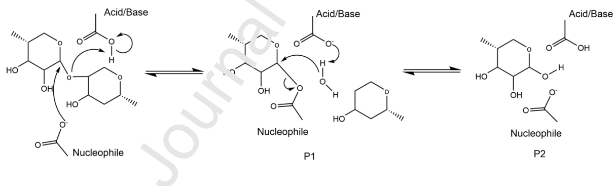
Figure 3. The Koshland double-displacement mechanism of \beta -mannanases as discussed by Sharma, Dhillon and Goyal [54]. P1 and P2 identify the reaction products.
