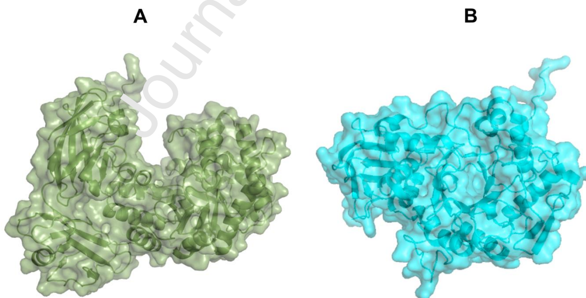
Figure 5. (A) Bacillus sp. BG-CS10 cellulase [87] (B) Halomonas meridiana \alpha -amylase [88]. Protein structures were predicted by AlphaFold ® and visualised with Pymol ® .
