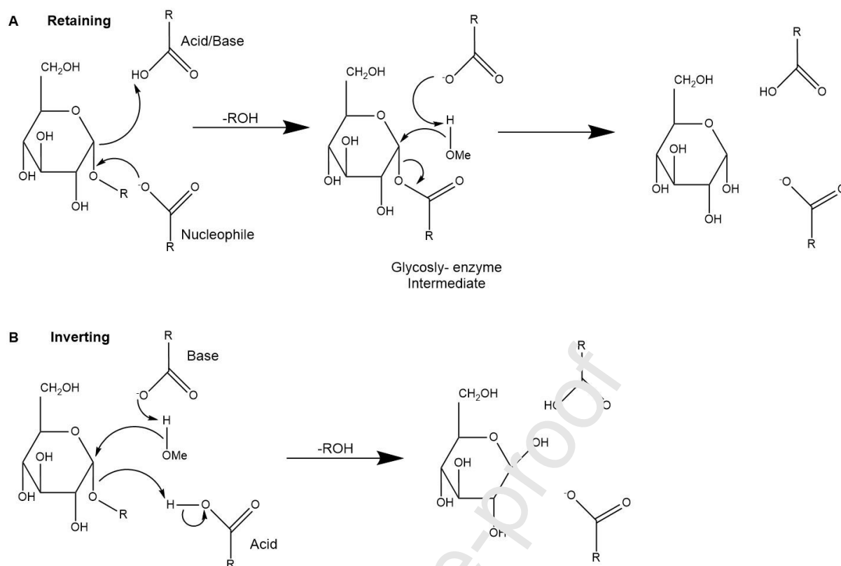
Figure 6. Mechanistic prediction of both retaining (A) and inverting (B) mechanism of \alpha -amylase with glutamate and aspartate residues as the acid/base and nucleophile respectively.
