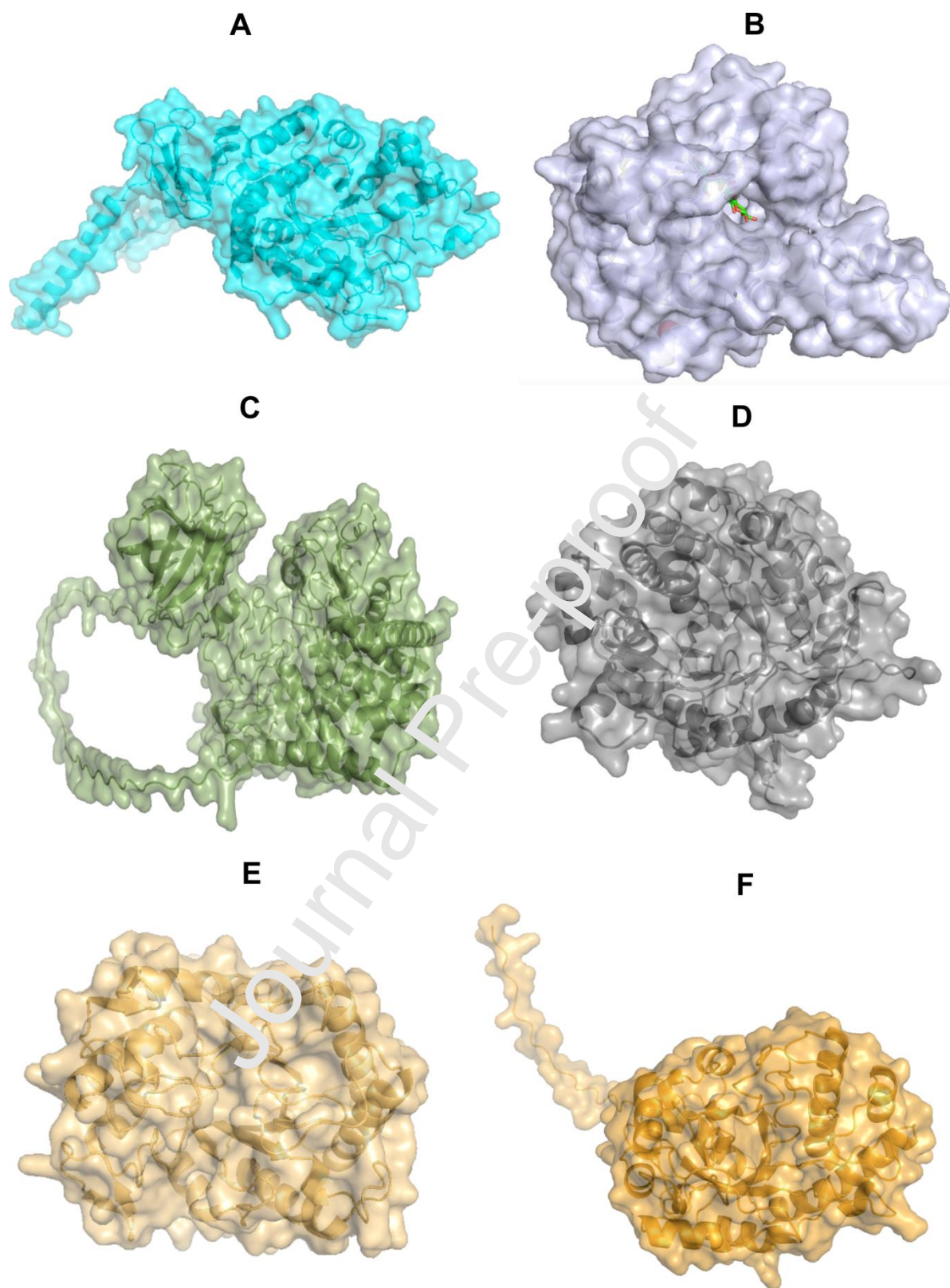
Figure 2. Structures of thermostable glycoside hydrolases for the degradation of starch, cellulose and hemicellulose. (a) Anoxybacillus sp. GXS-BL . \alpha -amylase. (b) Thermobifida fusca Cellobiohydrolase Cel6B (c) Spirochaeta thermophila
