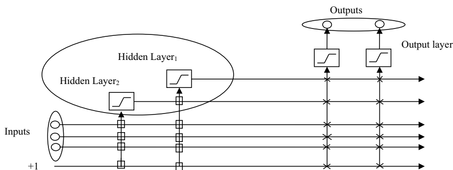
Fig. 5 Architecture of a cascade correlation network. As shown in this Figure, a Cascade Correlation network comprises an input layer, one or more hidden layers, and an output layer. The cascade architecture is characterized by its adaptive growth, where hidden neurons are introduced sequentially as the training progresses. Unlike traditional neural networks, where all hidden neurons are preset at the onset of training, in Cascade Correlation networks, once a neuron is added to the hidden layer, its incoming weights become frozen, ensuring that its pattern of activity is not modified in subsequent iterations. This dynamic architecture aids in the enhancement of the network’s capability and adaptability. The second foundational principle revolves around the learning process. When introducing a new neuron to the hidden layer, the training algorithm specifically aims to maximize the correlation between the output of this newly added component and the residual error of the network. This approach ensures that each added neuron makes a significant contribution towards correcting the overall network error, leading to efficient and effective training. This combination of dynamic architecture and specialized learning makes the Cascade Correlation network a powerful tool for various tasks. Source: Abdou, et al. (2016), pp. 91–92, Modified
