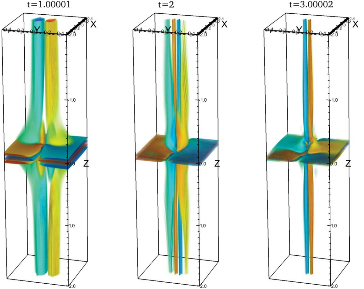
Figure 7. Vorticity tube formation about the spine and in the fan plane over time ( \omega \cdot \hat{B} ) (see also the supplementary movie). The vorticity is associated with propagating Alfvén waves.
