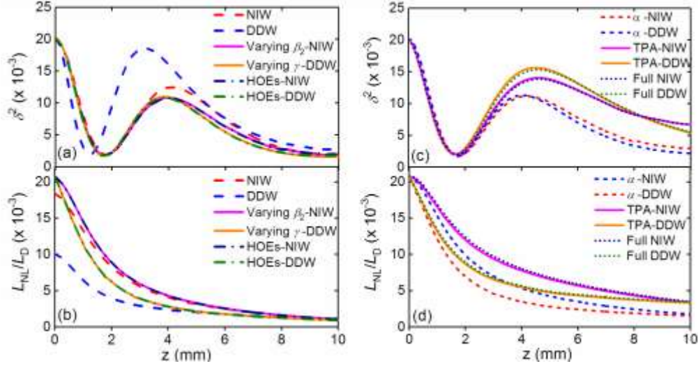
Fig. 8. (a) The mismatch factor \delta^2 and (b) ratio L_{NL}/L_D at 1550 nm for NIW (red dashed curves), DDW (blue dashed curves), varying \beta_2 -NIW (magenta solid curves), varying \gamma -DDW (orange solid curves), HOEs-NIW (navy dash-dotted curves) and HOEs-DDW (olive dash-dotted curves). (c) The mismatch factor \delta^2 and (d) ratio L_{NL}/L_D at 1550 nm for \alpha -NIW (blue dashed curves), \alpha -DDW (red dashed curves), TPA-NIW (magenta solid curves), TPA-DDW (orange solid curves), Full NIW (navy dash-dotted curves), and Full DDW (olive dash-dotted curves).
