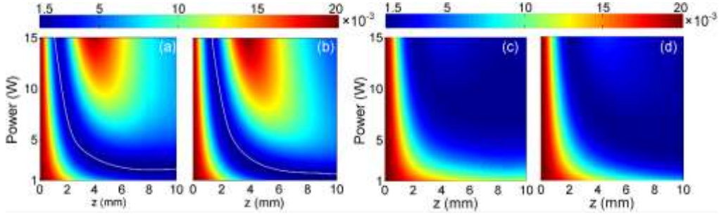
Fig. 11. The mismatch \delta^2 for (a) full NIW at 1550 nm, (b) full DDW at 1550 nm, (c) full NIW at 2150 nm and (d) full DDW at 2150 nm. The curves in white in (a) and (b) represent the minimum \delta^2 at each power P .
