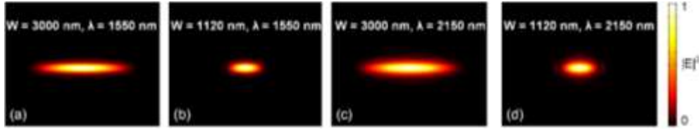
Fig. 3. Optical field distributions at (a) input port with W = 3000 nm and \lambda=1550 nm, (b) output port with W = 1120 nm and \lambda=1550 nm, (c) input port with W = 3000 nm and \lambda=2150 nm, and (d) output port with W = 1120 nm and \lambda=2150 nm.
