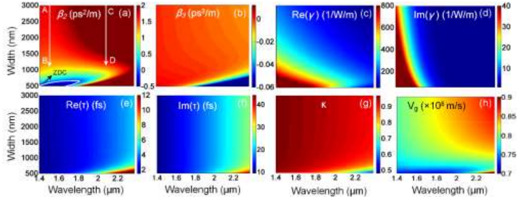
Fig. 2. The variation of (a) \beta_2 , (b) \beta_3 , (c) real part of \gamma , (d) imaginary part of \gamma , (e) real part of \tau , (f) imaginary part of \tau , (g) confinement factor \kappa , and (h) group velocity v_g as function of the wavelength and taper width.
