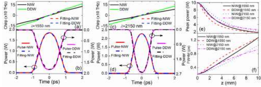
Fig. 5. (a) Chirp profiles (solid curves) and their linear fits (dashed curves) for NIW (black and red curves) and DDW (green and blue curves) at 1550 nm. (b) Output pulse waveforms (solid curves) and their parabolic fits (dashed curves) for NIW (red and magenta curves) and DDW (blue and black curves) at 1550 nm. (c) Chirp profiles (solid curves) and their linear fits (dashed curves) for NIW (black and red curves) and DDW (green and blue curves) at 2150 nm. (d) Output pulse waveforms (solid curves) and their parabolic fits (dash-dotted curves) for NIW (red and blue curves) and DDW (magenta and black curves) at 2150 nm. (e) The peak power of propagating pulses for NIW (black solid curves) and DDW (red dashed curves) at 1550 nm, and NIW (blue dotted curves) and DDW (magenta dash-dotted curves) at 2150 nm. (f) The FWHM of propagating pulses, for NIW (black solid curves) and DDW (red dashed curves) at 1550 nm, and NIW (blue dotted curves) and DDW (magenta dash-dotted curves) at 2150 nm.
