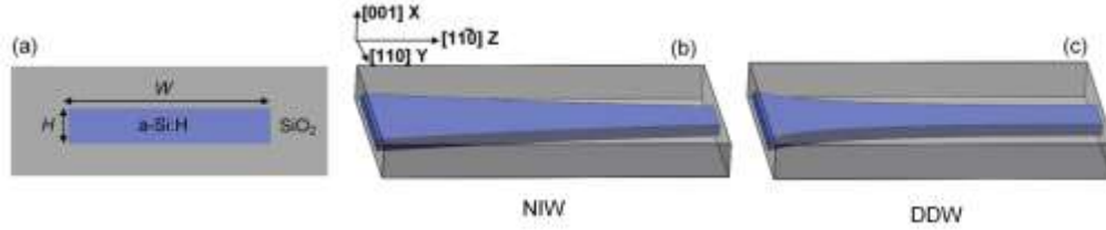
Fig. 1. Schematics of the (a) cross-section, and the three-dimensional view of (b) nonlinearity increasing and (c) dispersion decreasing tapered a-Si:H-PhWs.
