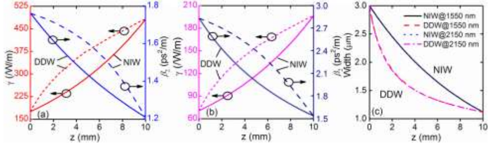
Fig. 4. Variations of nonlinear coefficient \gamma and dispersion \beta_2 in NIWs and DDWs with pump wavelengths at (a) 1550 nm and (b) 2150 nm. The solid curves are the designed parameters and the dashed curves are the corresponding parameters. (c) The taper width profile W(z) of NIWs and DDWs with pump wavelength 1550 nm and 2150 nm.
