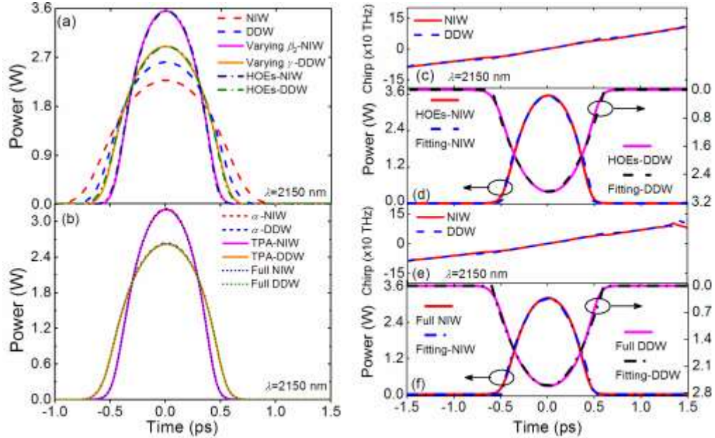
Fig. 9. Output pulses with pump wavelength 2150 nm. (a) Output pulse waveforms with ideal NIW (red dashed curve), ideal DDW (blue dashed curve), varying \beta_2 -NIW (magenta solid curve), varying \gamma -DDW (orange solid curve), HOEs-NIW (navy dash-dotted curve), and HOEs-DDW (olive dot-dashed curve), (b) Output pulse waveforms with
