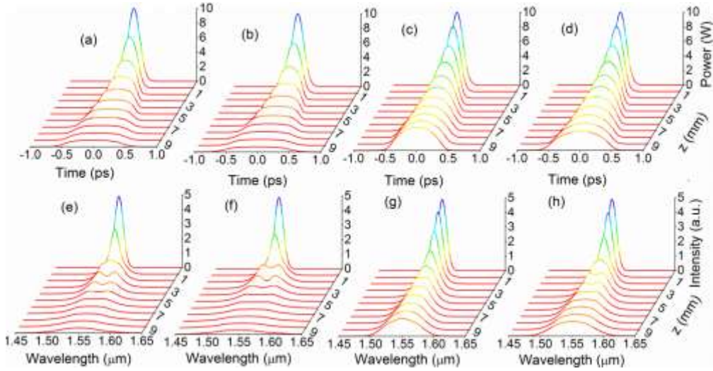
Fig. 6. Evolutions of the Gaussian input pulses along the taper modeled by the GNLSE. The evolutions of the waveforms in the top row are obtained in (a) NIWs at 1550 nm, (b) DDWs at 1550 nm, (c) NIWs at 2150 nm and (d) DDWs at 2150 nm. The evolutions of the spectra in the bottom row are obtained in (e) NIWs at 1550 nm, (f) DDWs at 1550 nm, (g) NIWs at 2150 nm and (h) DDWs at 2150 nm.
