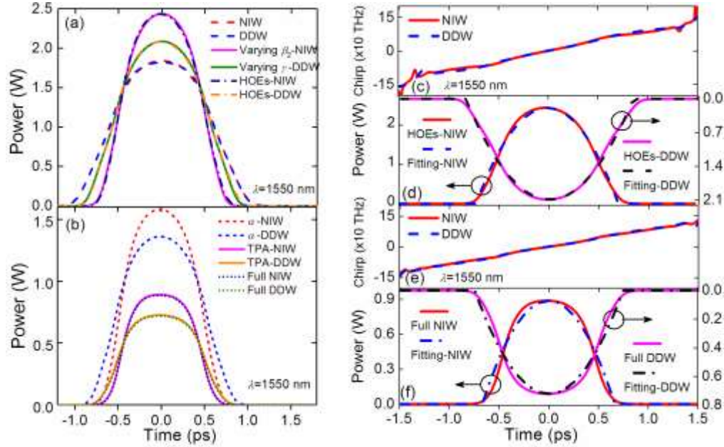
Fig. 7. Output pulses with pump wavelength 1550 nm. (a) Output pulse waveforms with ideal NIW (red dashed curve), ideal DDW (blue dashed curve), varying \beta_2 -NIW (magenta solid curve), varying \gamma -DDW (orange solid curve), HOEs-NIW (navy dash-dotted curve), and HOEs-DDW (olive dash-dotted curve), (b) Output pulse waveforms with lossy terms in \alpha -NIWs (red short dashed curve), \alpha -DDW (blue short dashed curve), TPA-NIW (magenta solid curve), TPA-DDW (orange solid curve), Full NIW (navy dotted curve) and Full DDW (olive dotted curve). (c) Chirp profiles of pulses from HOEs-NIW (red solid curves) and HOEs-DDW (blue dashed curve). (d) Output pulses of HOEs-NIW (red solid curve), parabolic fit for NIW (blue dashed curve), HOEs-DDW (magenta solid curve), and parabolic fit for DDW (black dashed curve). (e) Chirp profiles of pulses from Full NIW (red solid curve) and Full DDW (blue dashed curve). (f) Output pulses of Full NIW (red solid curve), parabolic fit for NIW (blue dash-dotted curve), Full DDW (magenta solid curve), and parabolic fit for DDW (black dash-dotted curve).
