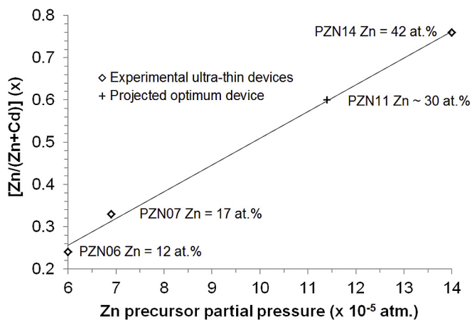
Fig. 8. The post-CdCl 2 Zn concentration (determined by XPS) as a function of Zn precursor partial pressure used in the MOCVD process to produce the Cd 1-x Zn x S window layer, showing projected Zn precursor partial pressure required to produce an ultra-thin device with [Zn/(Zn + Cd)] (x) fraction value = 0.6 for the Cd 1-x Zn x S window layer.
