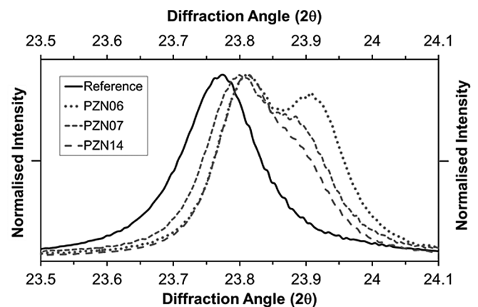
Fig. 5. XRD diffraction peaks of the CdTe (111) crystal plane showing variable \text{CdTe}_{1-y}\text{S}_y phase formation for ultra-thin PV cells with different \text{Cd}_{1-x}\text{Zn}_x\text{S} window layer Zn concentrations.
