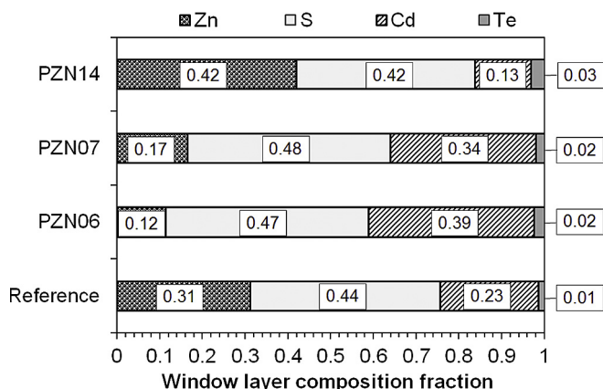
Fig. 2. Elemental fraction in the formed quaternary \text{Cd}_{1-x}\text{Zn}_x\text{S}_{1-y}\text{Te}_z alloy layer following \text{CdCl}_2 activation treatment and interdiffusion as determined by XPS.
