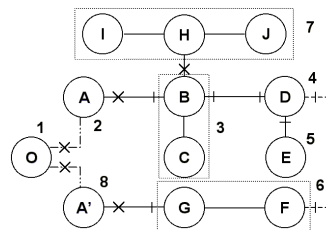
Figure 3. Graph associated with the electric system.
