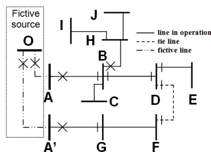
Figure 2. Initial test system.
