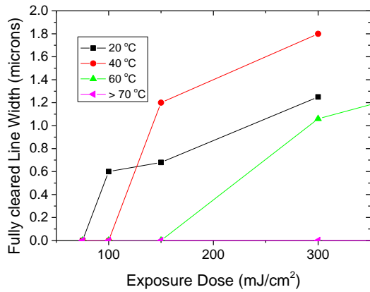
Figure 2 Examination of the patterned line width as a function of exposure dose for a range of bake temperatures.
