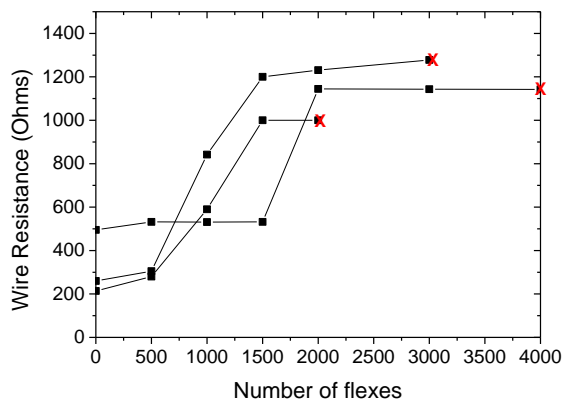
Figure 10 Automated cyclic testing of micro fabricated wires.
