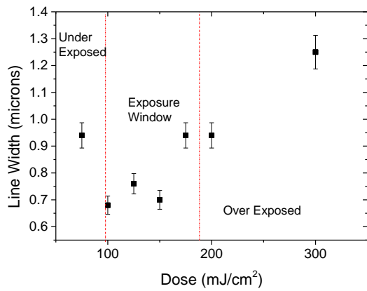
Figure 4 Dose test examination of feature line width on air dried samples.
