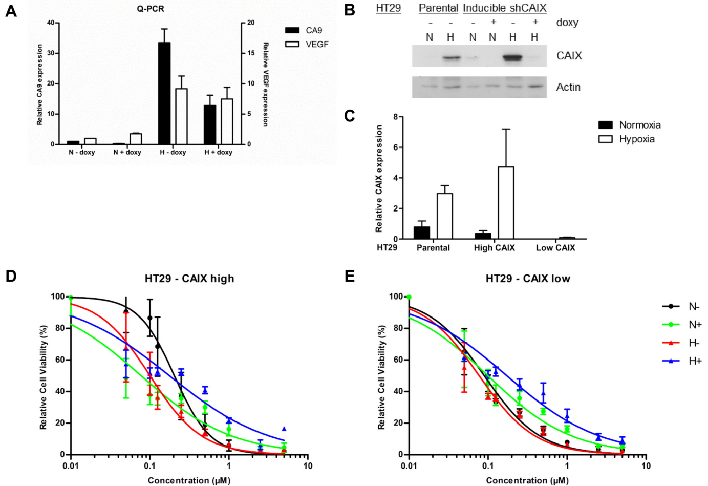
Fig 2. Effect of S4 on doxorubicin efficacy in HT29-CAIX high and HT29-CAIX low cells. Exposing HT29 cells to doxycycline (doxy) reduced CA9 mRNA levels during normoxia (N) and hypoxia (H), whereas VEGF levels were unaffected (A). CAIX protein levels minimized in HT29-CAIX low cells when exposed to doxycycline (B). Quantification of three independent biological repeats showed minimal residual CAIX protein expression in HT29-CAIX low cells as compared to parental cells or HT29-CAIX high cells without a KD (C). Cell viability assays of HT29-CAIX high (D) or HT29-CAIX low cells (E) with increasing concentrations of doxorubicin. Cells were exposed to vehicle (black) or S4 (green) during normoxia (N), or to vehicle (red) or S4 (blue) during hypoxia (H). Results of three independent biological repeats are shown (mean ± SEM).
