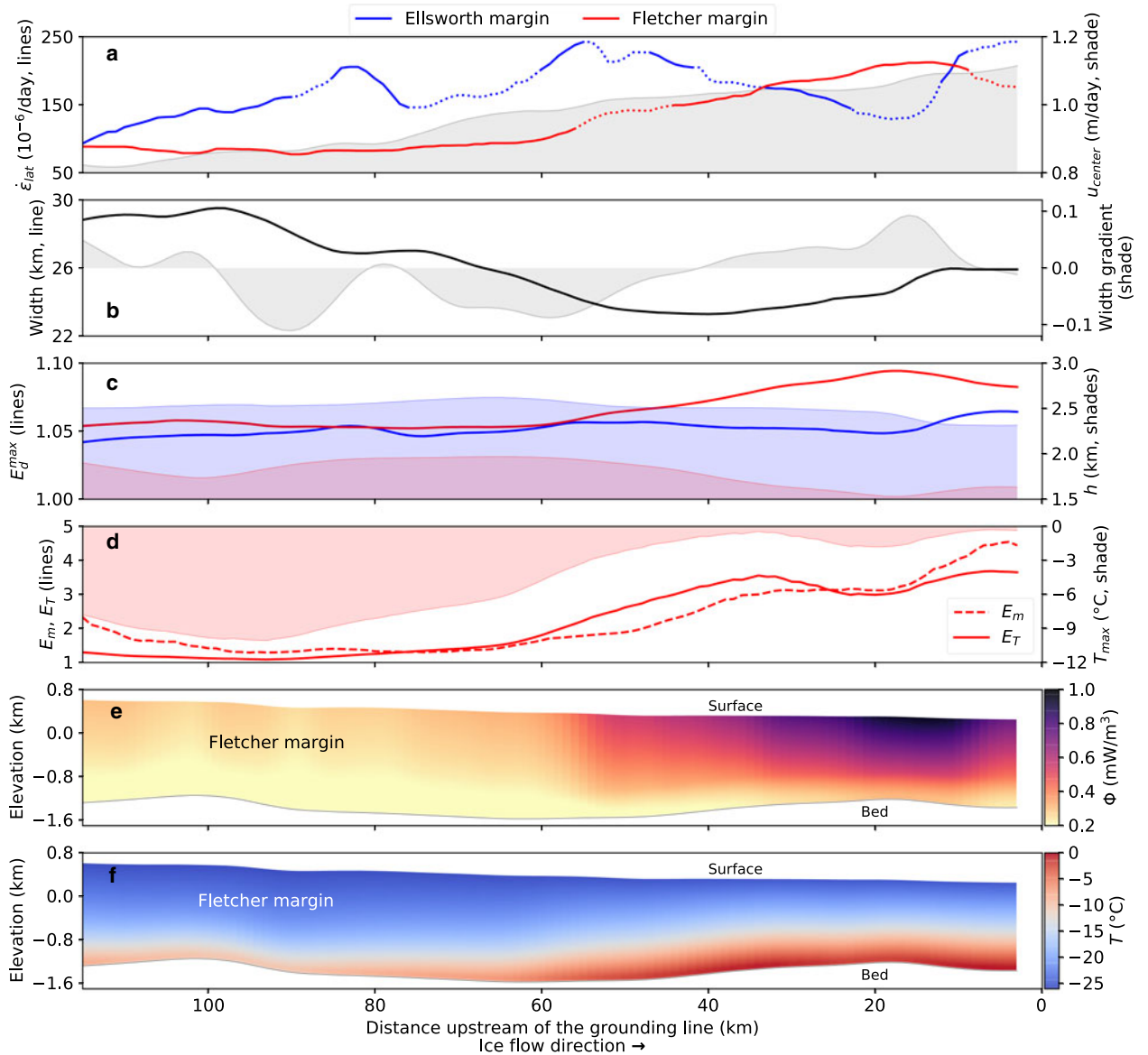
Fig. 3. Along-flow variations in the Ellsworth (blue) and Fletcher (red) margins of RIS. (a) Lateral shear strain rates (lines) and horizontal speed along the centerline (gray shade). Dashed line segments occur where tributary glaciers intersect RIS (Fig. 1b). (b) Total RIS width (black line) and along-flow gradient of width (gray shade). We define width to be the distance between strain-rate maxima in each margin (Fig. 2b). (c) Maximum macroscopic-damage enhancement factor E_d^{\max} (lines) and ice thickness h in the margins (shaded regions). (d) Thermal, E_T , (solid line) and margin, E_m , (dashed line) enhancement factors overlaying inferred maximum (basal) ice temperature (shaded region). All values for E_T and T are calculated using E_i A^* = 18 (see Table 1 for A^* values). (e) Steady-state rates of shear heating, \Phi , and (f) ice temperature with elevation defined relative to mean sea level. For reference, 1 \text{ mW/m}^3 \approx 16.7 \times 10^{-3} \text{ }^\circ\text{C a}^{-1} , using values given in Table 1. We show only the Fletcher margin in (d–f) because ice thickness is poorly constrained in the Ellsworth margin.
