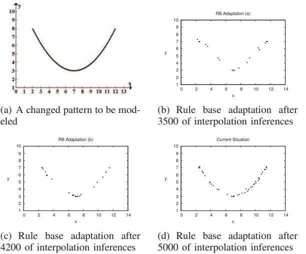
Fig. 6. The processes of rule base adaptation
