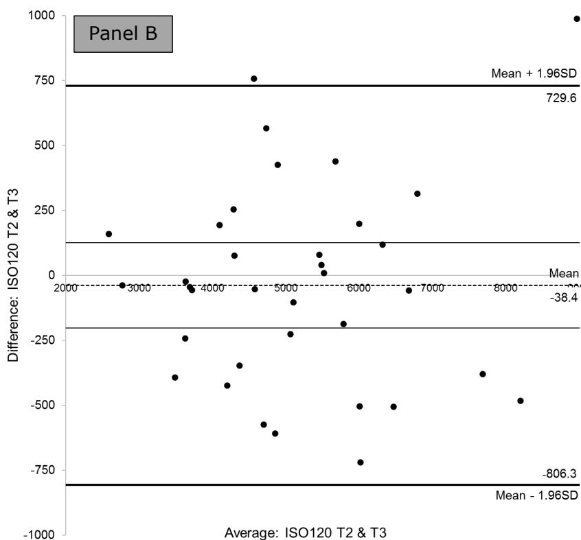
Figure 2. Bland-Altman plot for ISO 90 (Panel A) and ISO 120 (Panel B). Dotted line represents calculation bias (mean difference). Thin solid lines represent calculation precision (95% confidence intervals). Thick solid lines represent the upper and lower limits of agreement.
