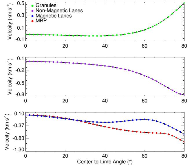
Figure 6. The RV of the four granulation components relative to disc centre as a function of limb angle.
