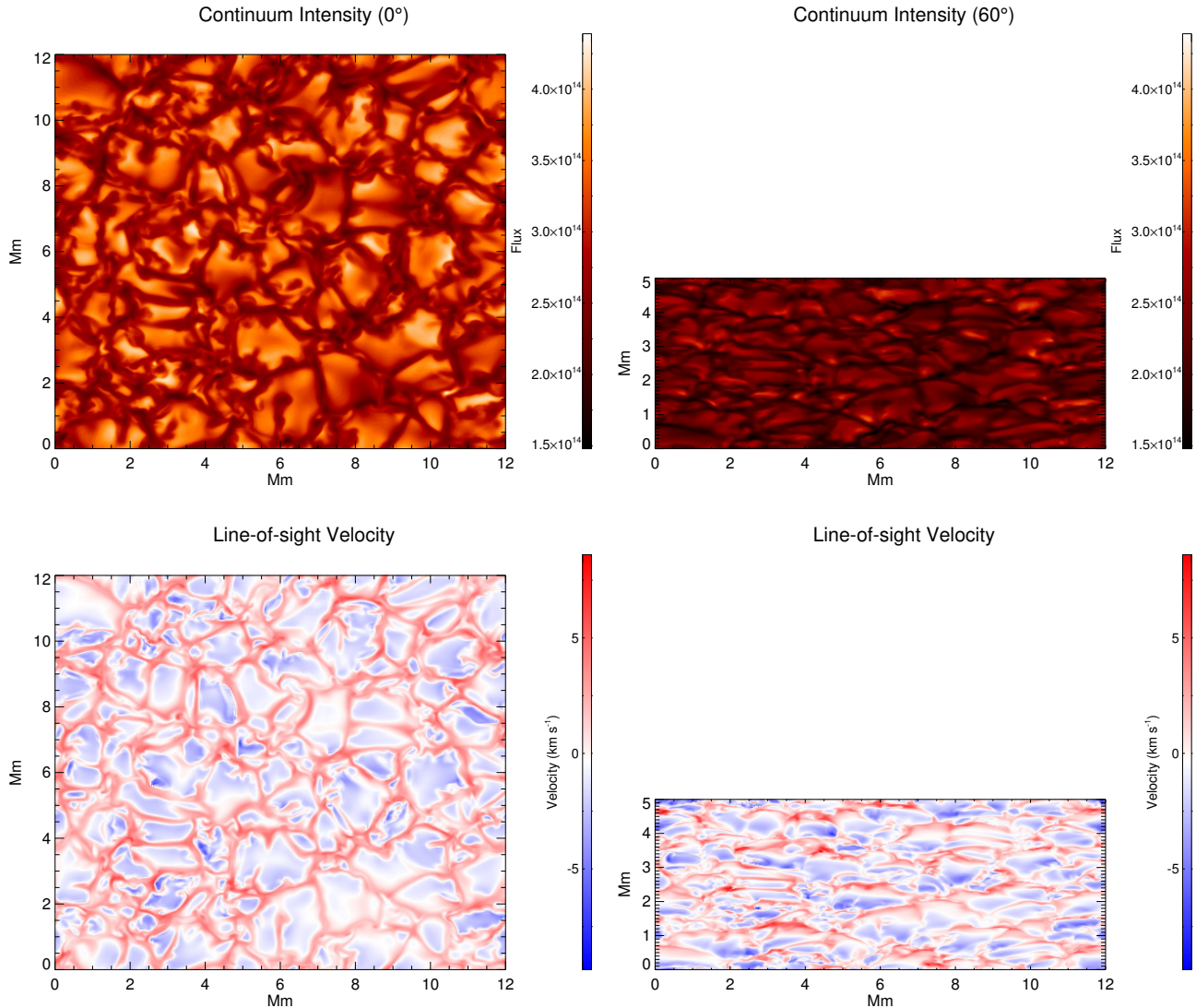
Figure 1. Continuum intensities (top) and line-of-sight velocities (bottom) for one simulation snapshot at two different stellar disc centre-to-limb angles: 0^\circ (left) and 60^\circ (right). Negative and positive velocities denote blueshifts and redshifts, respectively.
