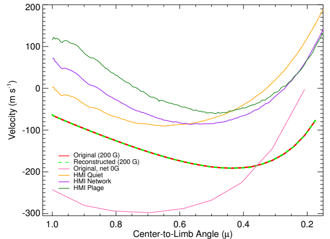
Figure 14. The net RV as a function of limb angle, calculated via the first moment. Profiles from the simulation were convolved with the instrumental profile of HMI (thick lines indicate the 200 G simulation). The Fe I 6173 Å HMI observations are separated into contributions from the quiet photosphere, facular network, and plage regions (with increasing magnetic field respectively) and are relative to the quiet Sun.
