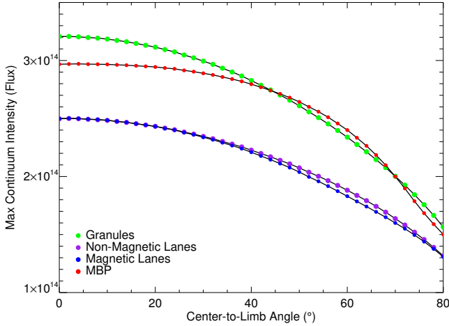
Figure 5. The maximum continuum intensity of the four granulation components as a function of limb angle; note the magnetic and non-magnetic intergranular lanes values are nearly identical. The initial near constant brightness of the MBP component may be due to inclusion of faculae.
