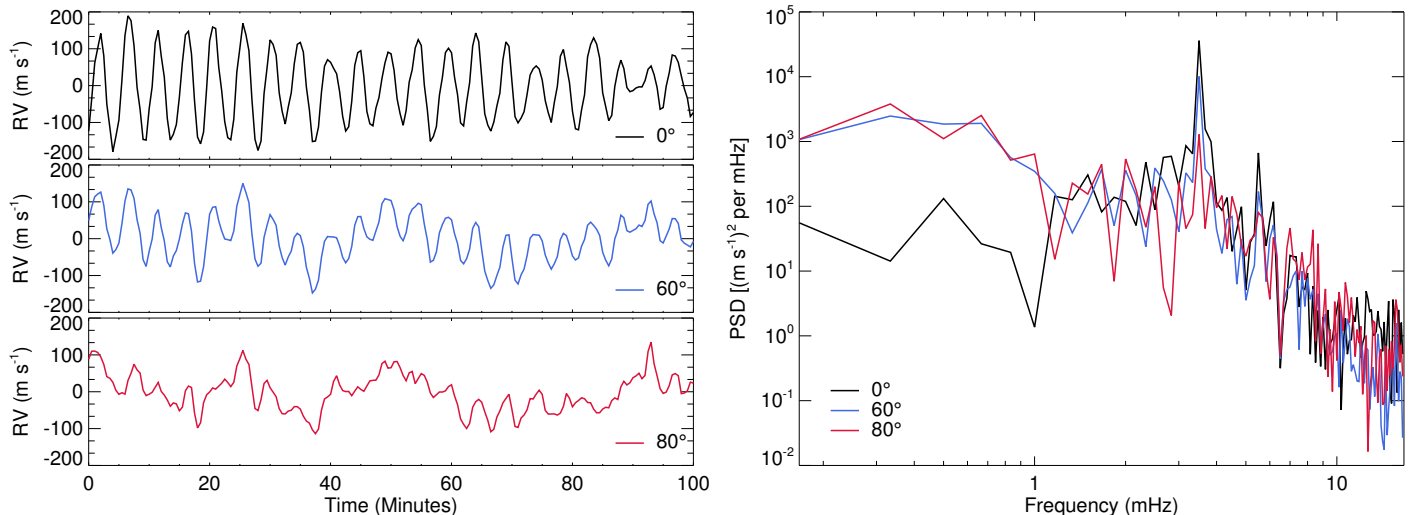
Figure 3. Original RVs from the average line profiles from each snapshot over the time-series (left) and their corresponding power spectra (right) for limb angles 0^\circ , 60^\circ , 80^\circ ; these include contributions from both p-mode oscillations and granulation.
