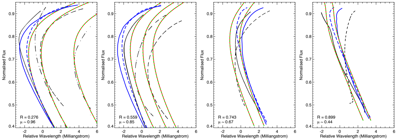
Figure 11. Time-average bisectors from the MHD simulation (red are from the original profiles and dashed green lines are from the reconstruction) for various centre-to-limb positions (denoted in units of solar radii and approximate \mu ), after convolution with an instrumental profile matching Cavallini et al. (1985a). Observations from Cavallini et al. (1985a) are shown in solid black lines for the quiet Sun and dashed/dot-dashed lines for facular regions; observations from Löhner-Böttcher et al. (2018) for the quiet Sun are shown in blue at \mu intervals of 0.1; dashed lines indicate \mu lower by 0.1. The simulated profiles and data from Löhner-Böttcher et al. (2018) have been shifted to various positions to ease shape comparison with Cavallini et al. (1985a).
