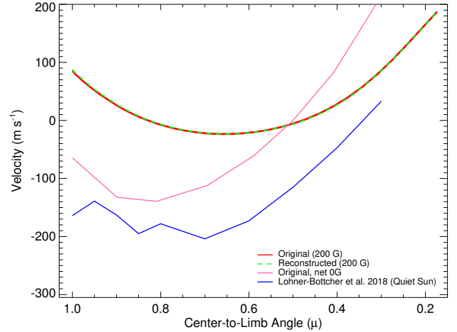
Figure 13. The net RV as a function of limb angle, calculated via a parabolic fit to the bottom of the line profile core. Profiles from the simulations were convolved with the instrumental profile from the LARS spectrograph (thick lines indicate the 200 G simulation).
