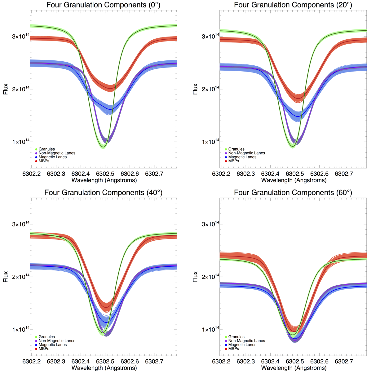
Figure 4. Average (thick) and individual (thin) line profiles from the four different contributions to granulation used in the parameterisation: granules (green), MBPs (red), magnetic (blue) and non-magnetic (purple) intergranular lanes, for four different stellar disc centre-to-limb angles. Flux is measured in units of \text{erg s}^{-1} \text{cm}^{-2} \text{sr}^{-1} \text{\AA}^{-1} .
