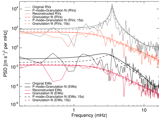
Figure 8. The power spectra, at disc centre, of the RVs and equivalent widths from the original and reconstructed line profiles; the equivalent width data has been scaled by a factor of 10^{-3} for viewing ease. Solid lines display an interpolation onto a 30 s cadence and dashed lines for a 15 s cadence; thick lines are the fits to the data (thin lines).
