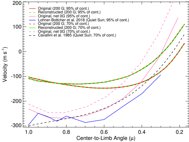
Figure 12. The net RV as a function of limb angle, calculated via the mean bisector up to either 70% or 95% of the continuum, and convolved with the corresponding instrumental profile; thick lines indicate the 200 G simulation.
