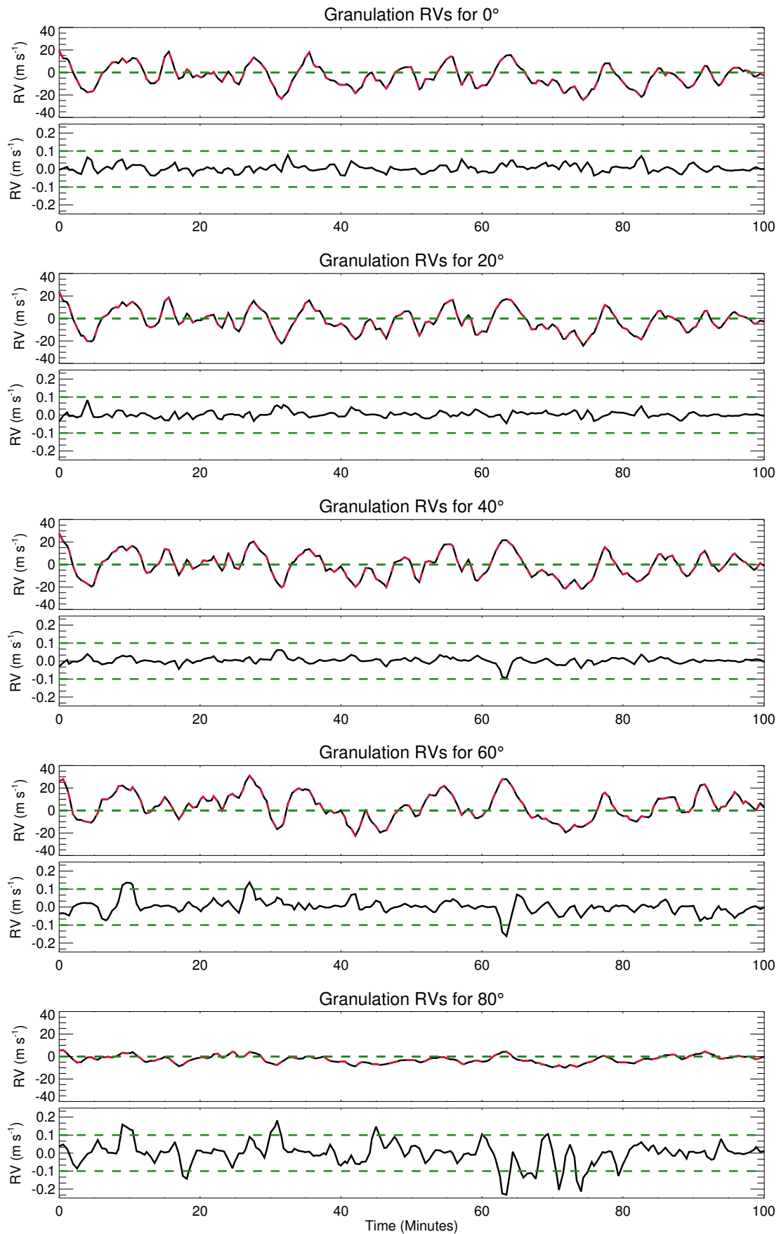
Figure 10. The granulation RVs from the simulation (original - oscillation) are shown in black, and those from the reconstruction are shown in dashed red lines, for various centre-to-limb angles; residuals between the two are also shown in black solid lines below. Horizontal dashed lines at \pm 10 \text{ cm s}^{-1} are provided to guide the eye.
