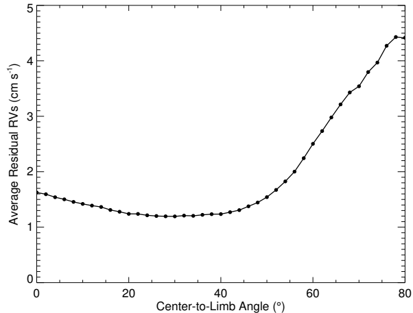
Figure 9. The average residual (original - reconstructed) RVs of the time-series as a function of limb angle.
