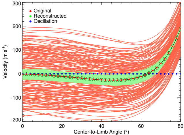
Figure 2. Net RVs relative to disc centre for both individual snapshots (lines) and averages over the time-series (points); original profile results are in red, connected by a solid black line, and the reconstructed (granulation-only) profiles are in green (see Sec. 3 and 4 for details). Scatter from individual profiles is due to p-modes and granular evolution (reconstruction only includes granular effects). Also plotted are the oscillation RVs averaged over the entire series (blue points), and a black dotted line at 0 \text{ m s}^{-1} to guide the eye.
