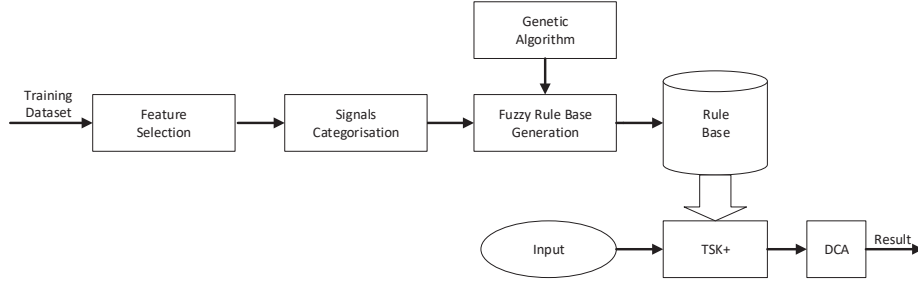
Fig. 1. The overall TSK-DCA system
