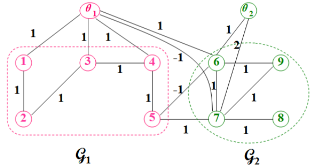
Fig. 3. Communication topology for Example 2.
