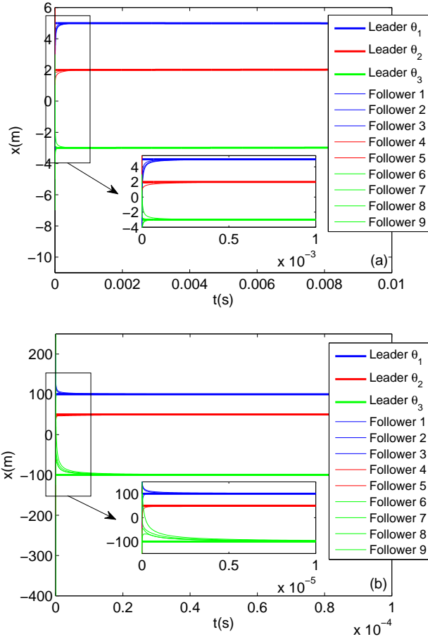
Fig. 2. Fixed-time group tracking consensus for multi-agent systems (3), (13) and communication topology shown in Example 1. (a) is for (x_{\theta_1}(0), x_{\theta_2}(0), x_{\theta_3}(0), x_1(0), x_2(0), x_3(0), x_4(0), x_5(0), x_6(0), x_7(0), x_8(0), x_9(0)) = (5, 2, -3, 2, -4, -3, 6, 0, -5, 3, 1, -7) ; and (b) is for (x_{\theta_1}(0), x_{\theta_2}(0), x_{\theta_3}(0), x_1(0), x_2(0), x_3(0), x_4(0), x_5(0), x_6(0), x_7(0), x_8(0), x_9(0)) = (100, 50, -100, -50, 200, 150, -200, 75, -125, -400, 250, 100) .
