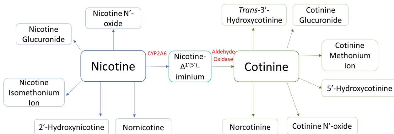
Figure 1.7. Overview of Nicotine and Cotinine metabolism and their associated metabolites. The main enzymes involved in nicotine metabolism are shown in red: Cytochrome P450 Family 2 Subfamily A Member 6 (CYP2A6) and Aldehyde Oxidase.
