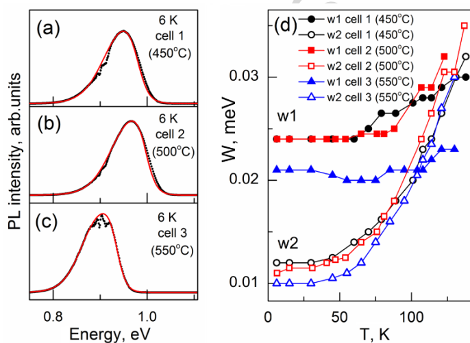
Fig. 5. The PL spectra (shown by symbols) of solar cell 1 (a), 2 (b) and 3 (c), taken at 6 K, fitted with asymmetric double sigmoidal functions (shown by red solid lines), Temperature dependence of fitting parameters W1 and W2 (d).
