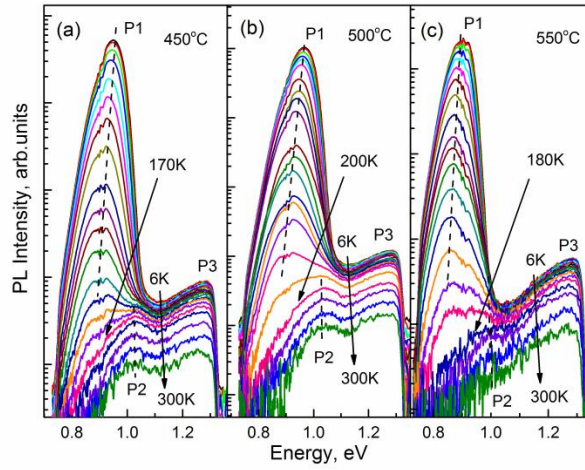
Fig. 4. Temperature dependencies of the PL spectra of the solar cells with the selenisation temperature of 450°C (a), 500°C (b) and 550°C (c).
