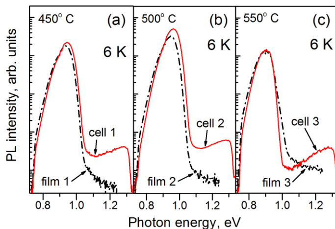
Fig. 8. A comparison of the PL spectra measured at 6 K in as deposited CZTSe films 1, 2 and 3, selenised at 450°C (a), 500°C (b), 550°C (c), respectively, and solar cells 1, 2 and 3 fabricated from these films.
