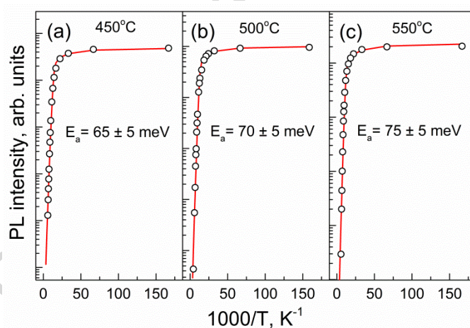
Fig. 7. Arrhenius plots of the integrated intensities of the FB bands in the PL spectra of solar cells 1(a), 2 (b) and 3(c).
