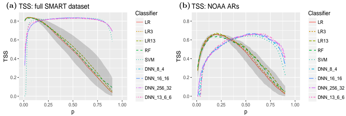
Figure 3. TSS or median TSS curve for all the classifiers. LR (LR with 3 features trained on subsamples), LR3 (LR with 3 features trained on the full training set), LR13 (LR with all features trained on the full training set), RF, SVM and four DNN architectures. TSS curve for LR (full line) has 2.5th and 97.5th percentile band. (a) Full SMART dataset, (b) NOAA AR dataset.
