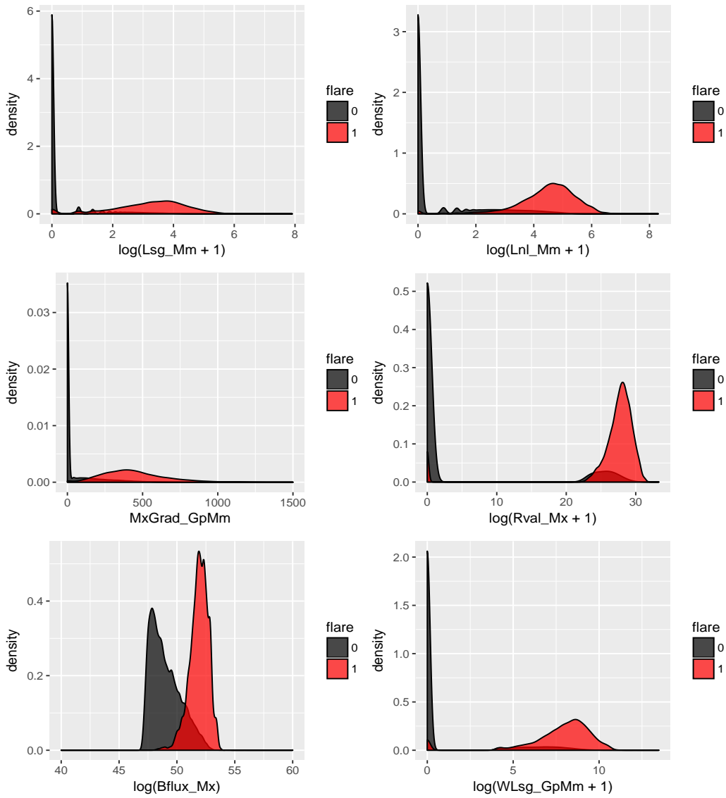
Figure 5. The marginal densities of the top features in the full SMART dataset selected by MR, Lasso and RF algorithms.
