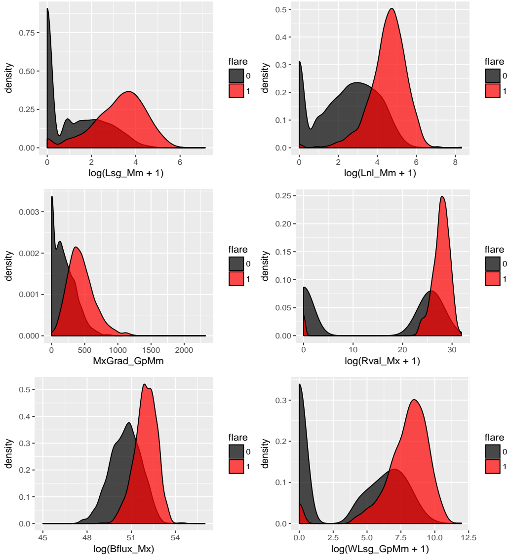
Figure 6. The marginal densities of the top features in the NOAA AR dataset selected by MR, Lasso and RF algorithms.
