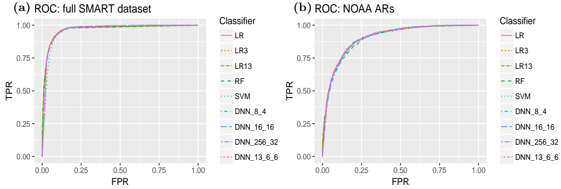
Figure 1. ROC curves, calculated for the training set for LR (LR with 3 features trained on subsamples), LR3 (LR with 3 features trained on the full training set), LR13 (LR with all features trained on the full training set), RF, SVM and the DNN architectures. (a) Full SMART dataset, (b) NOAA ARs dataset.
