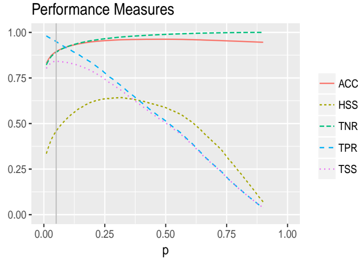
Figure 2. Sensitivity (TPR), specificity (TNR), accuracy, TSS and HSS over a range of probability thresholds. Estimated probability was obtained from the logistic regression with three features on the full SMART dataset. The proportion of flares in the training dataset is 0.05 (vertical line).
