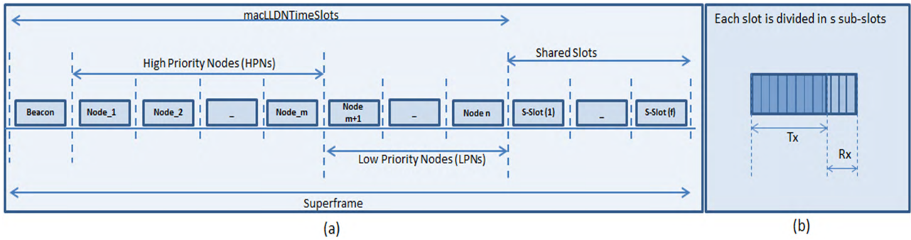
FIGURE 3. Superframe ( n < 20 ).
