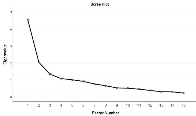
Figure 1. Scree Plot
