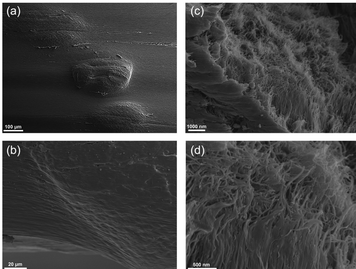
Figure 7. FE-SEM images of fractured surface with appearance of dark bands of agglomerated nanotubes: (a) and (b) elevated regions/bumps at lower magnification; (c) Agglomerates of nanotubes visible beneath the surface of elevated regions; and (d) higher resolution image showing clear agglomerates of nanotubes.
