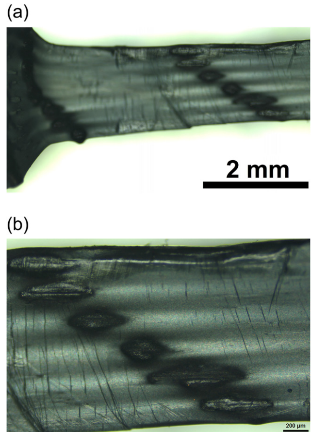
Figure 5. Representative 2D Optical microscopic images for 1wt% HDPE nanocomposites. Clear bright translucent (matrix) and dark (agglomerated nanotubes) bands are visible in both images.
