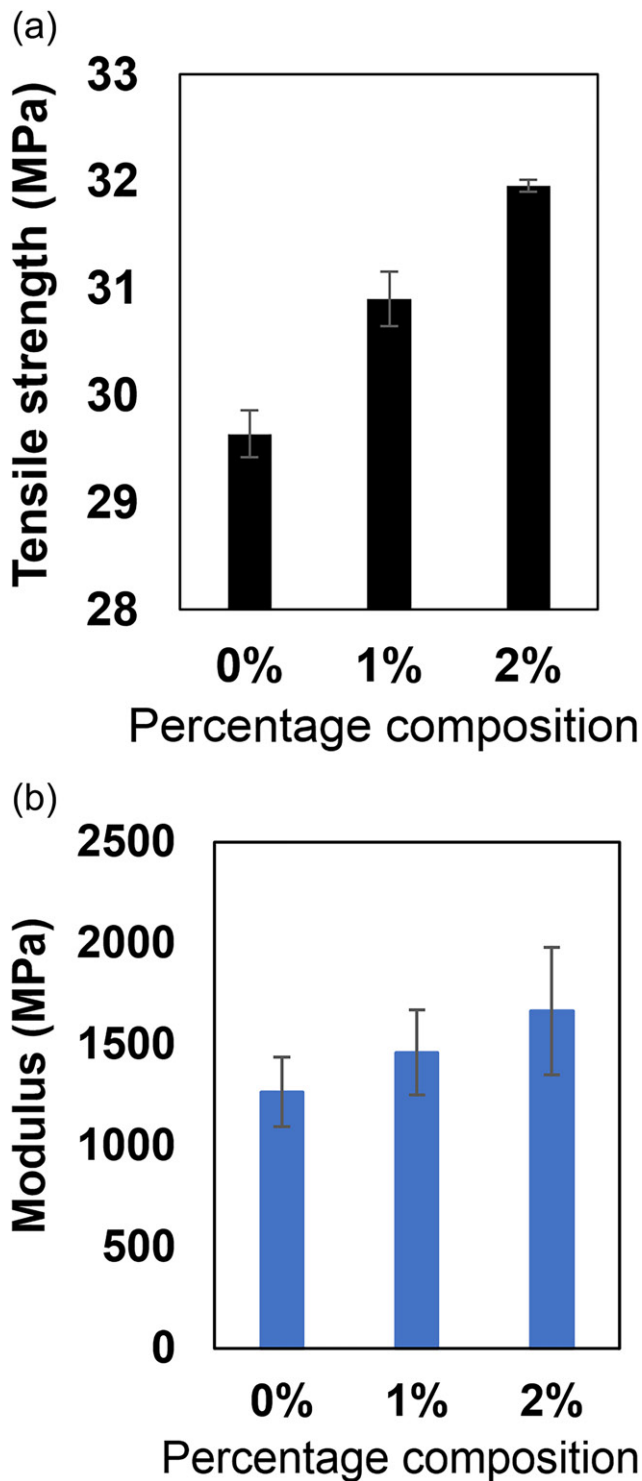
Figure 2. Mechanical properties of various HDPE nanocomposite compositions: (a) tensile strength; and (b) modulus.
