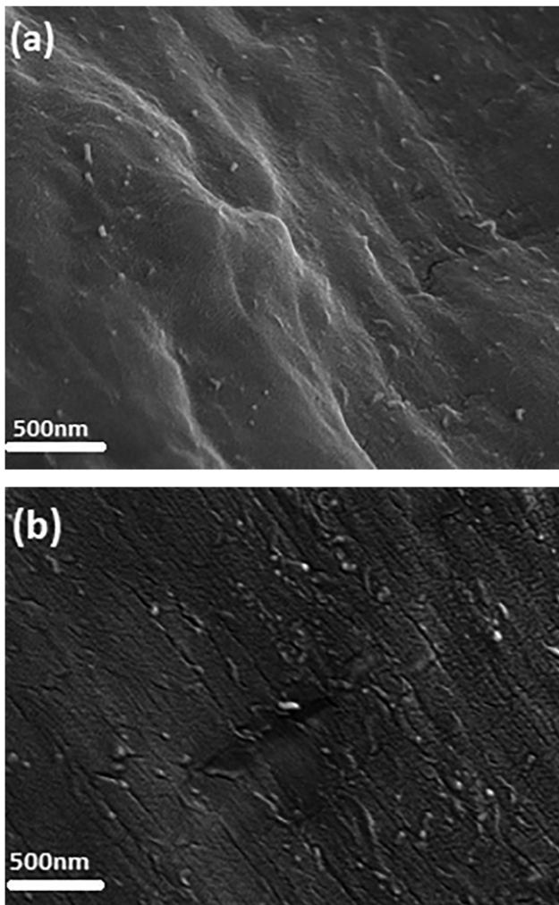
Figure 3. FESEM image showing state of dispersion at HDPE-1CNT (a) and HDPE-2CNT (b).
