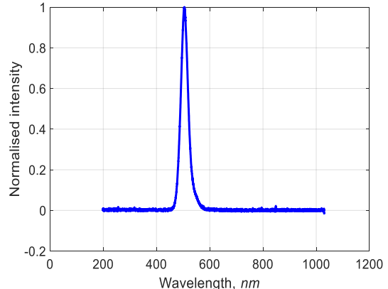
Fig. 4. The measured spectral wavelength for green traffic light (a peak wavelength of 504.7 nm).
