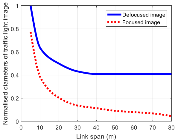
Fig. 6. The normalised diameter of traffic light image with reference to the defocused mode versus link span
