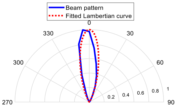
Fig. 3. The normalized beam profile of green traffic light
