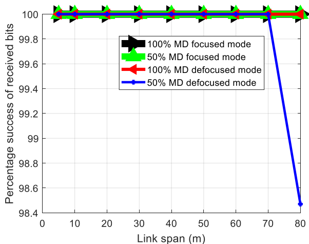
Fig. 7. Success rate of the data transmission over a link span for the focused and defocused camera modes
