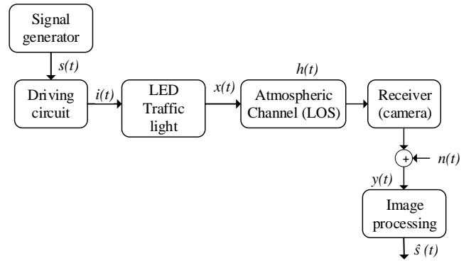
Fig. 1. The schematic block diagram of a VLC-based V2I system.
