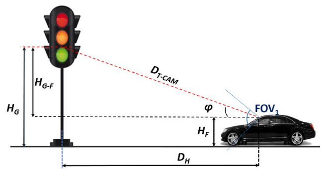
Fig. 2. Configuration of the V2I VLC system
