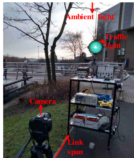
Fig. 5. The experimental setup for the V2I VLC system
