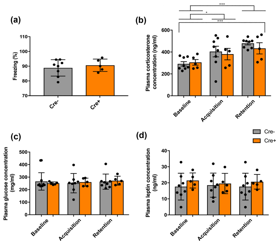
Fig. 6 Freezing behavior and blood plasma analysis of HPA-axis biomarkers performed on ChAT::Cre+ ( n = 5 ) and ChAT::Cre- ( n = 8 ) rats at baseline (2 days before initiating the task protocol), with testing that was then repeated at the fear acquisition and fear retention stages of a CFCT. a Freezing scores acquired for retention testing; b comparison of corticosterone blood plasma levels between genotypes at the different CFCT testing phases; c a similar comparison made for glucose blood plasma levels and for d leptin blood plasma
