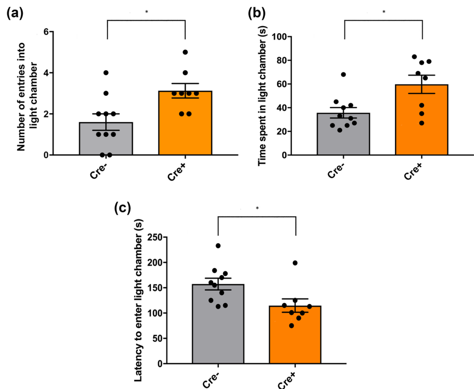
Fig. 3 The LDB is another conventional anxiety test that is based on the innate aversion of rodents to brightly illuminated areas, which was utilized to test unconditional anxiety responses in the rats. The ChAT::Cre+ rats ( n = 8 ) showed a greater preference for the light compartment of the box compared to their ChAT::Cre- siblings ( n = 10 ). Behavioral parameters assessed were: a total number of entries made into the light chamber, b time spent in the light chamber and c latency time for rats to enter the light chamber. All data are presented as the mean \pm SEM. * p \leq 0.05 , compared to ChAT::Cre- rats
