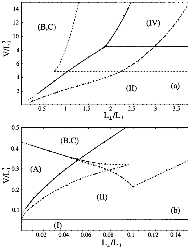
FIG. 6. (a) Bifurcation diagram for liquid morphologies on two lyophilic stripes within a lyophobic substrate as a function of the reduced separation L_{\perp}/L_1 between the two stripes and of the reduced volume V/L_1^3 ; and (b) a more detailed view of the same bifurcation diagram for small values of L_{\perp} and V . In both figures, the contact angles are \theta_{\gamma}=30^{\circ} on the lyophilic stripes and \theta_{\delta}=120^{\circ} on the lyophobic substrate. Dashed lines are instability lines whereas full lines represent the loci of morphological transitions. Bridge morphologies connecting the two stripes are denoted by (A), (B), and (C) as in Fig. 5. For sufficiently large separation L_{\perp} , these bridges rupture, and the liquid forms a channel state (II) or a bulge state (IV) on one of the two lyophilic stripes as in Fig. 1.
