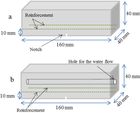
Figure 2. Typical prism: (a) for water absorption test and (b) for water flow test. Table 2 presents the number of specimens that were used per test in each laboratory.
