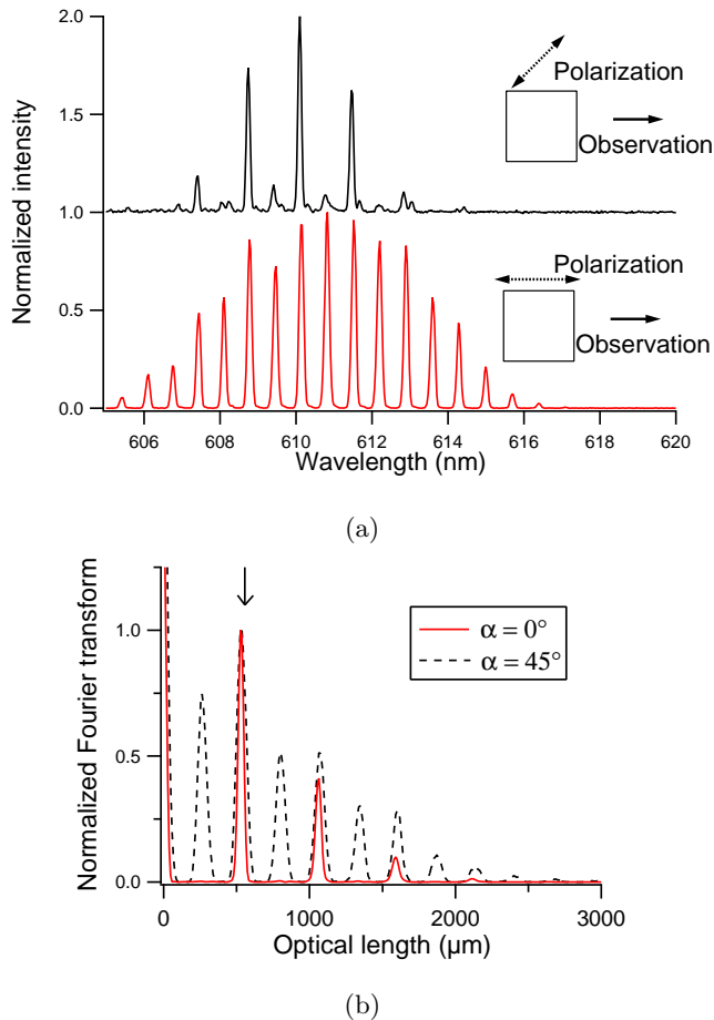
FIG. 8: (Color online) (a) Experimental spectra from a square micro-laser with a = 120 \mu\text{m} . Top: \alpha = 45^\circ , bottom: \alpha = 0^\circ . (b) Fourier transform of the spectra in (a). The arrow indicates the predicted optical length of the diamond periodic orbit: 2\sqrt{2}an .
