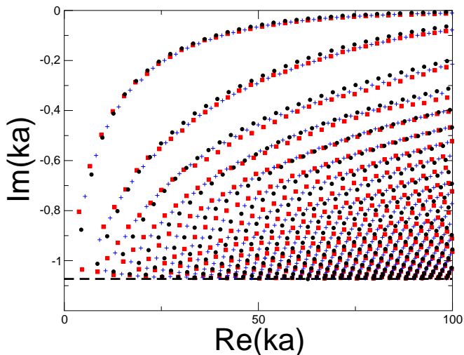
FIG. 3: (Color online) Resonance spectrum for the dielectric square with n = 1.5 . The crosses, squares, and circles correspond respectively to (-+) , (++) , and (--) symmetry classes. The position of the horizontal dashed line is given by (13).
