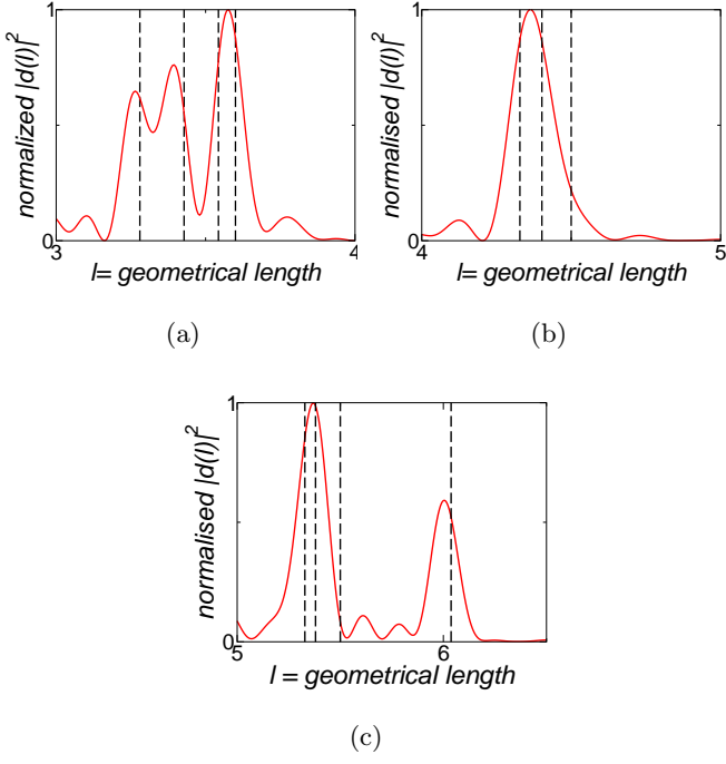
FIG. 25: Length densities calculated from numerical spectra for dielectric stadiums with (—) symmetry class and n = 1.5 . (a) \rho = 0.3 . (b) \rho = 0.75 . (c) \rho = 1.25 . The vertical dotted lines indicate the expected positions of periodic orbits (numbering according to Fig. 26).
