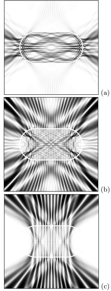
FIG. 24: Wave functions of the dielectric stadium with \rho = 1 , (- -) symmetry class, and n = 1.5 . (a) kR = 34.48 - 0.11 i . (b) kR = 34.55 - 0.31 i . (c) kR = 34.48 - 0.45 i . Greyscale, black representing maximal values of |\psi|^2 .
