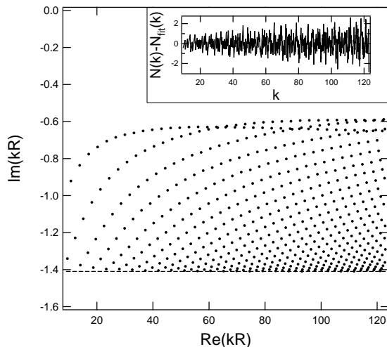
FIG. 6: Resonance spectrum for the dielectric square with n = 1.35 and (--) symmetry class. The positions of the horizontal dashed lines are given by (13). Insert: N(k) - N_{fit}(k) with a = 1 .
