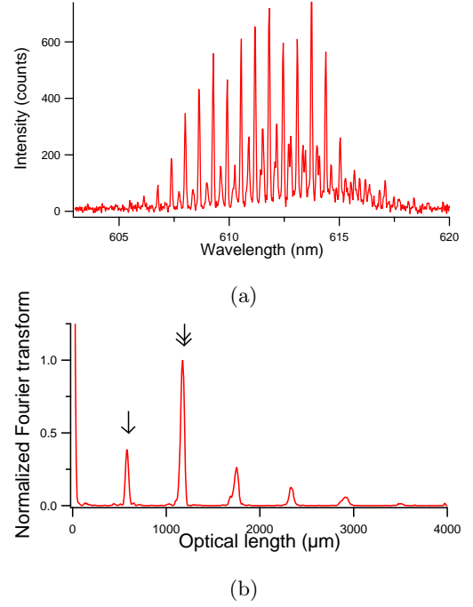
FIG. 22: (a) Experimental spectrum from a pentagonal microlaser with a = 90 \mu\text{m} . (b) Fourier transform of the spectrum in (a). The single (resp. double) arrow indicates the expected position of the single (resp. double) pentagon periodic orbit.
