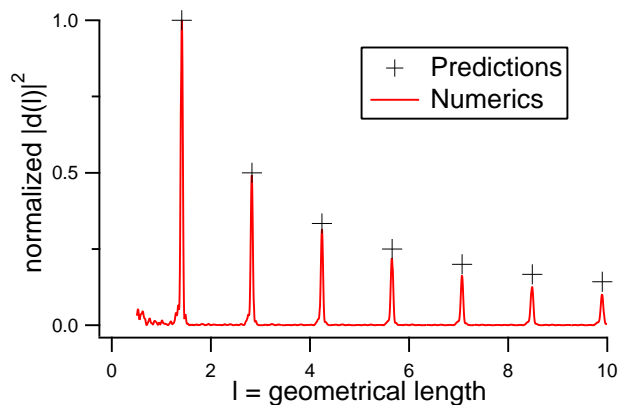
FIG. 7: Comparison of |d(l)|^2 calculated from the numerical data of the dielectric square for (--) symmetry class and n = 1.5 (continuous line), and predictions from trace formula (crosses) considering the m^{\text{th}} repetitions of half the diamond periodic orbit ( l = ma\sqrt{2} ) with a coefficient |d(l)|^2 \propto 1/m .
