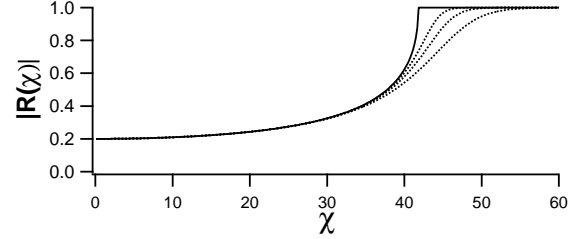
FIG. 29: Modulus of the TM reflection coefficient as a function of the incidence angle (in degrees). Full line: Fresnel coefficient (10) for a straight boundary. Dotted lines: (24) for kR = 100, 50, 25 .
