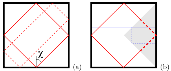
FIG. 2: (a) Two representations of the same diamond periodic orbit. Definition of the incident angle \chi . (b) The dashed part corresponds to the fundamental domain used for numerical simulations. The Fabry-Perot and diamond periodic orbits are drawn, as well as their restriction to the fundamental domain (dotted lines).
