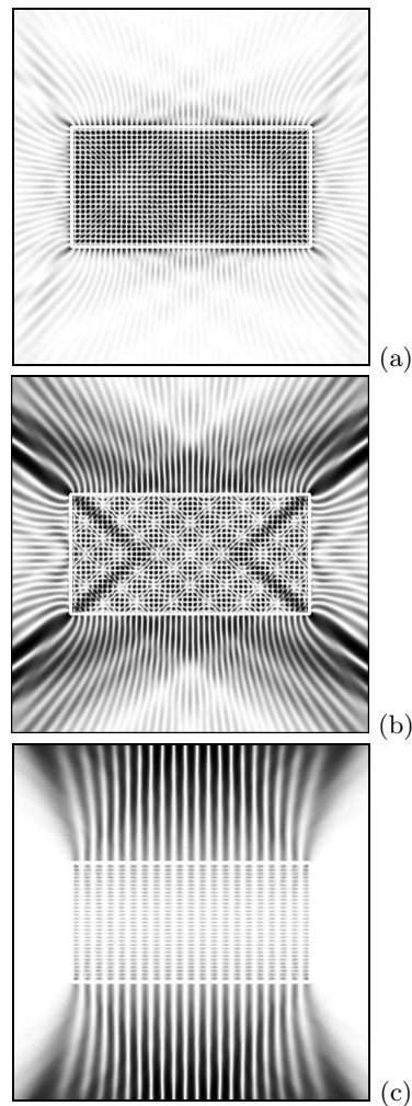
FIG. 12: Quasi-stationary states for the dielectric rectangle, n = 1.5 , (++) symmetry class. (a) kl = 70.04 - .038i , (b) kl = 70.26 - .33i . (c) kl = 70.45 - .92i . Greyscale, black representing maximal values of |\psi|^2 .
