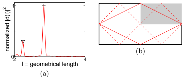
FIG. 11: (a) Length density for a dielectric rectangle calculated from the spectrum in Fig. 9. The expected position of the double diamond (resp. the stretched diamond) is indicated by a cross (resp. a triangle). (b) Main periodic orbits contributing to the resonance spectrum: double diamond (dashed line) and stretched diamond (continuous line). The dashed area corresponds to the fundamental domain.
