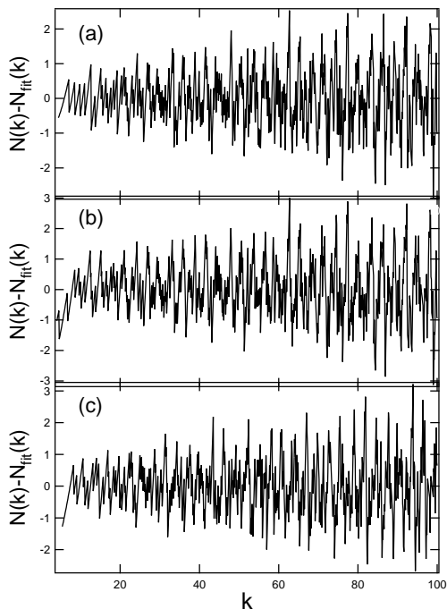
FIG. 5: Residue N(k) - N_{fit}(k) for the dielectric square ( a = 1 ) with n = 1.5 and different symmetry classes : (a) (--) , (b) (++) , and (c) (-+) .
