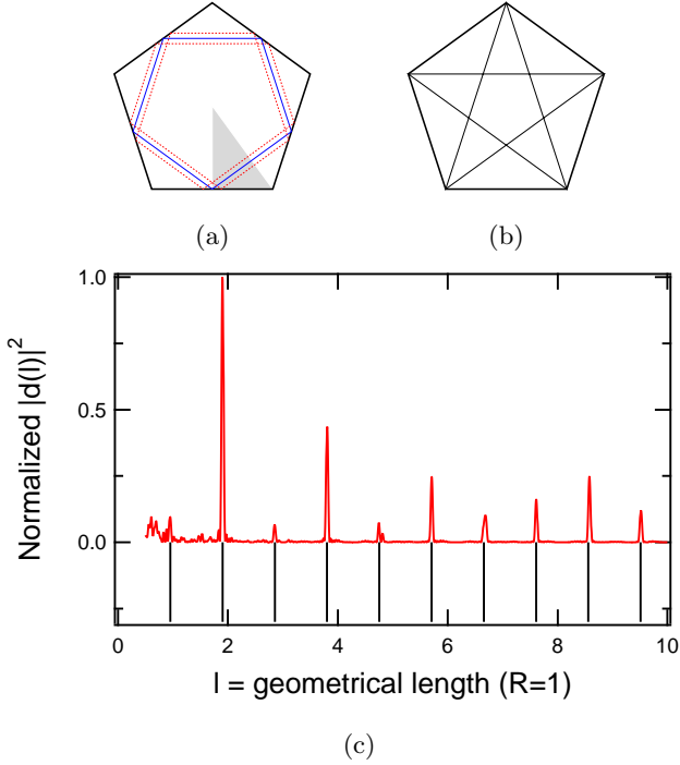
FIG. 20: (Color online) (a) 'single pentagon' periodic orbit in solid line and 'double pentagon' periodic orbit in dotted line. The dashed area indicates the fundamental domain used for simulations. (b) A representation of the double pentagon periodic orbit. (c) Length density for the dielectric pentagon calculated from the numerical data plotted in Fig. 18a. The vertical lines in the bottom part of the graph indicate the repetitions of the single pentagon orbit.
