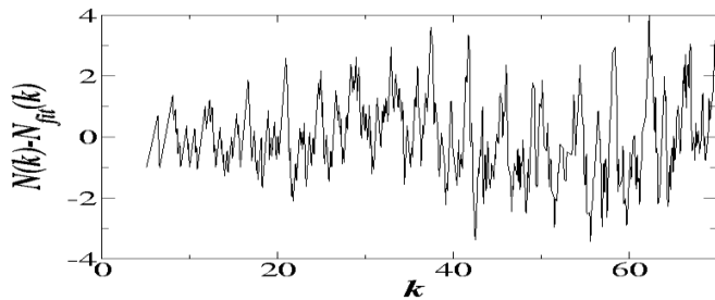
FIG. 10: Residue N(k) - N_{fit}(k) for the dielectric rectangle with \rho = 2 , l = 1 , (++) symmetry class, and n = 1.5 .
