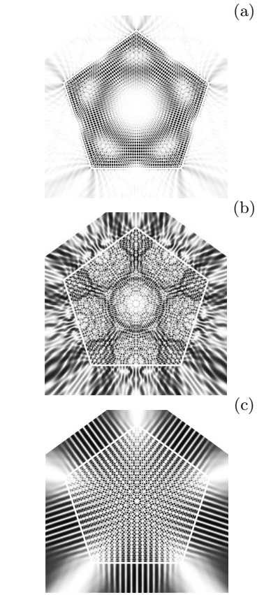
FIG. 19: Wave functions of the dielectric pentagon with (- -) symmetry and n = 1.5 . (a) kR = 91.35 - 0.038i , (b) kR = 89.06 - 0.453i , and (c) kR = 92.56 - 0.628i . Greyscale, black representing maximal values of |\psi|^2 .
