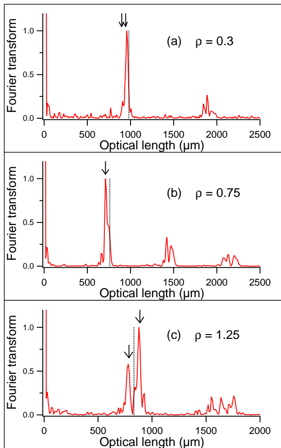
FIG. 31: Normalized Fourier transform of experimental spectra from stadium micro-lasers with (a) R = 80 \mu m , (b) R = 50 \mu m , and (c) R = 45 \mu m . The vertical line corresponds to the position of the perimeter. The arrows indicate the expected positions of some orbits, for comparison: (a) orbits 1 and 2, (b) orbit 1, and (c) orbits 1 and 5 (numbering according to Fig. 26).
