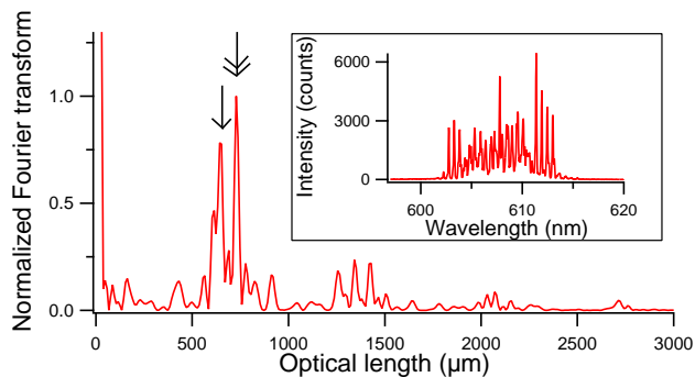
FIG. 17: Fourier transform of the spectrum in insert. The arrows indicate the predicted optical length of periodic orbits: single arrow for the Fabry-Perot along the major axis 4an and double arrow for the rectangle 4bn\sqrt{1+\rho^2} . Insert: Experimental spectrum from an elliptical micro-laser with \rho = a/b = 2 and b = 50 \mu\text{m} registered in the direction parallel to the major axis.
