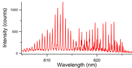
FIG. 30: Experimental spectrum of a stadium micro-laser with \rho = 0.75 and R = 50 \mu m . Its Fourier transform is plotted in Fig. 31b.
