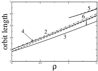
FIG. 27: Geometrical length of the periodic orbits plotted in Fig. 26. Numbering according to Fig. 26.
