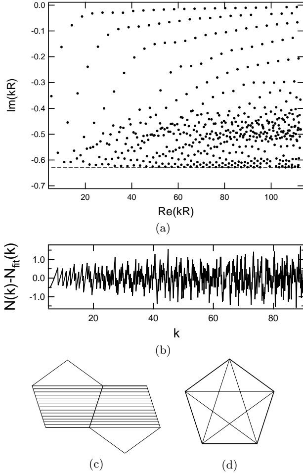
FIG. 18: (a) Resonance spectrum for the dielectric pentagon with (- -) symmetry and n = 1.5 . The position of the horizontal dashed line is given by (20). (b) N(k) - N_{fit}(k) calculated from the numerical spectrum in (a) with R = 1 . (c) A part of the periodic orbit with the shortest lifetime. (d) A representation of the periodic orbit in (c).
