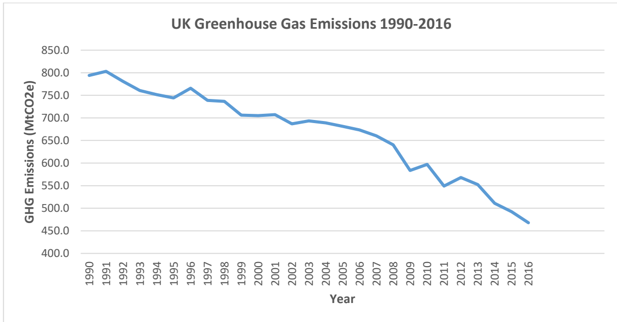
Fig 2 - GHG emissions national statistics 1990-2016 (BEIS., 2018b)
