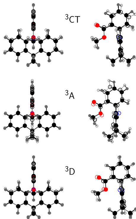
Figure 12: Deformations of DMAC-MB in different optimized C_s symmetric triplet geometries, as annotated. The deformations with respect to the C_s ground state geometry have been multiplied by a factor of 5. The deformed geometries (open circles, grey bonds) are superimposed to the ground state geometry (filled circles, black bonds).
