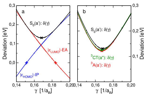
Figure 10: Determination of range separation parameter \gamma for optimized geometries in different electronic configurations respecting C_s mirror symmetry. (a) for S_0(a') configuration, (b) comparison of optimized geometries in the configurations S_0(a') , {}^3\text{CT}(a'') , and {}^3\text{A}(a') , evaluated in the electronic ground state S_0 . For each data point (dots), the geometry has been optimized in the respective electronic configuration. Colored lines are based on cubic polynomials fitted to |\epsilon_{\text{HOMO}}| - \text{IP} and |\epsilon_{\text{LUMO}}| - \text{EA} . For the latter two, zero crossings are marked (+), together with the minimum of \delta(\gamma) (x).
