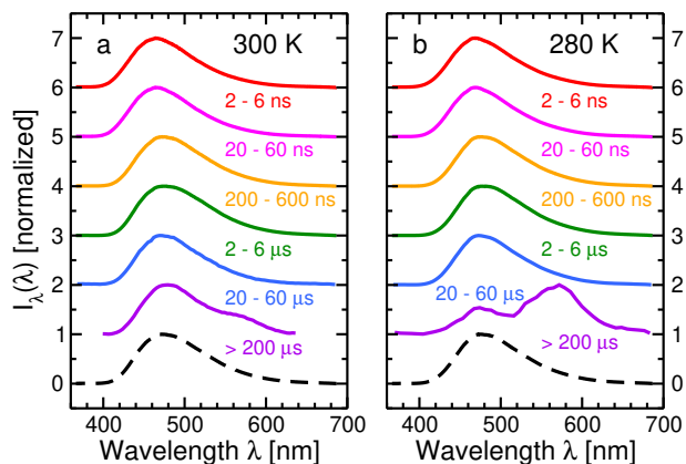
Figure 5: Fluorescence spectra I_{\lambda}(\lambda) of a film containing 5 wt.% DMAC-MB embedded in zeonex, integrated over different delay intervals, at temperatures of (a) T = 300 K and (b) T = 280 K. For clarity, each spectrum is normalized to its peak value and shifted vertically, from top to bottom: delay 2 ns to 6 ns (red), 20 ns to 60 ns (magenta), 200 ns to 600 ns (orange), 2 \mu s to 6 \mu s (green), 20 \mu s to 60 \mu s (blue), and time integration from 200 \mu s to 2 ms (purple). At each temperature, the time-integrated spectrum (from 2 ns to 2 ms) is shown as a black dashed line.
