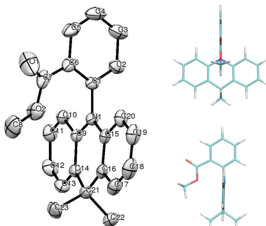
28 29 30 31 32 33 34 35 36 37 38 39 40 41 42 43 Figure 1: Left: ORTEP view (50% probability level) of the DMAC-MB structure in the 44 crystalline phase, drawn using Mercury software. H-atoms have been omitted for clarity. 45 Right: C_s symmetric geometry of free DMAC-MB, optimized with an optimally tuned range- 46 separated hybrid functional, seen along the normal of the DMAC donor group (top), and 47 along the normal of the MB acceptor group (bottom). 48 49 50
