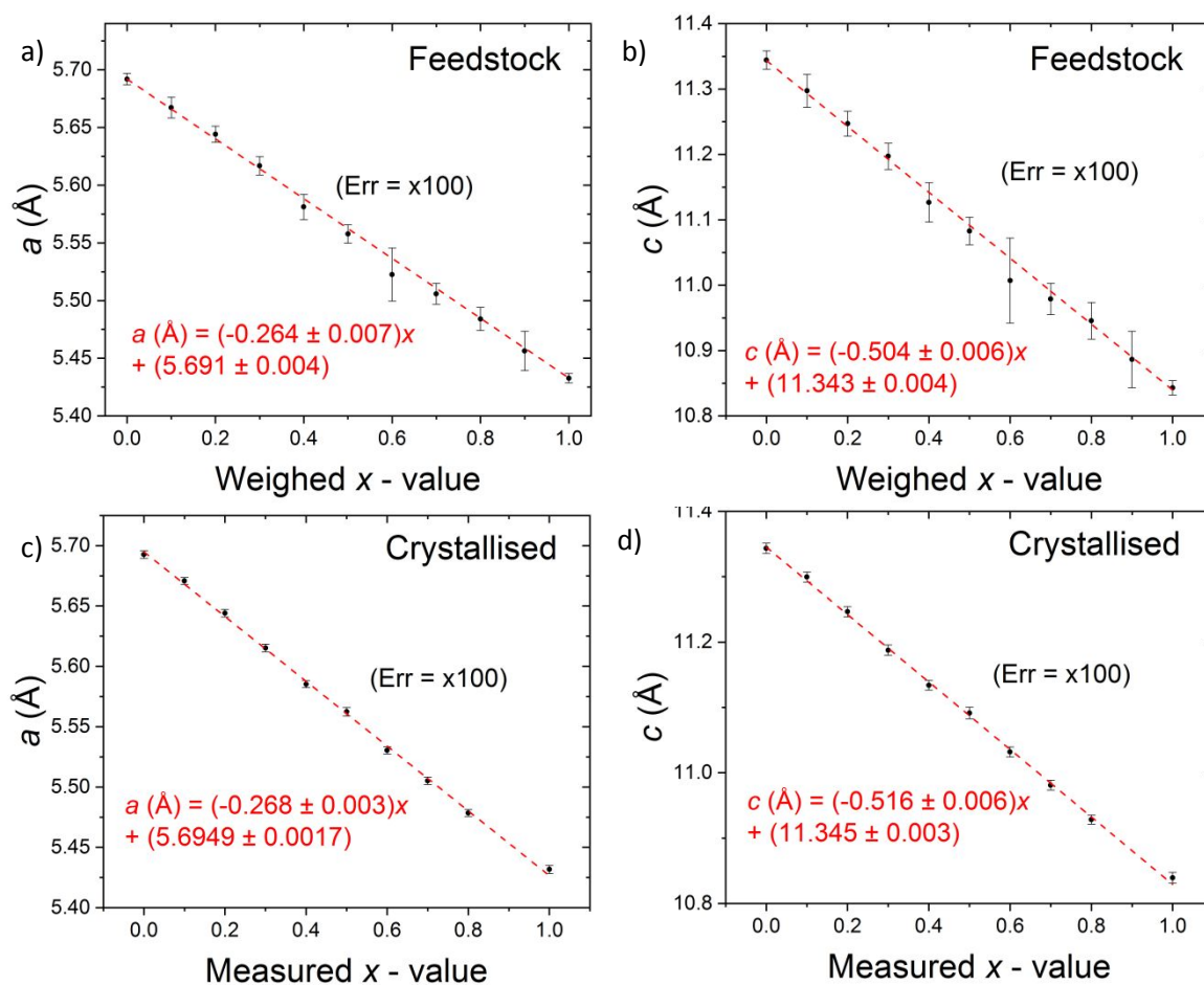
Figure 4. Lattice parameters a and c for \text{Cu}_2\text{ZnSnS}_{4x}\text{Se}_{4-4x} ( 0 \leq x \leq 1 ). Data for the as-synthesised feedstock are shown in (a) and (b) respectively, (weighed x values) and for the crystallised materials in (c) and (d), with x values based on the elemental ratios measured with ICP-OES (see Table S1). The values were extracted from the XRD patterns by Rietveld refinement. Both sets of samples show linear Vegard relationships, indicating that solid-solutions are formed. The equations of the best linear fits are shown on the graphs. The error bars displayed on all plots are 100x larger than the real uncertainties on the lattice parameter values, in order to allow comparison of the uncertainty between data points.
