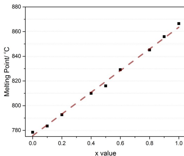
Figure 1. Melting points of \text{Cu}_2\text{ZnSnS}_{4x}\text{Se}_{4-4x} feedstock as a function of weighed sulfur fraction x measured using differential scanning calorimetry at a heating rate of 5^\circ\text{C} .
