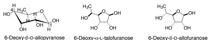
Figure 2: 6-Deoxy- \beta -D-allopyranose in a ^4\text{C}_1 conformation and 6-deoxy- \alpha -L-talofuranose and 6-deoxy- \beta -D-allofuranose
