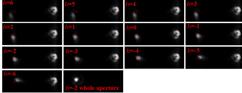
Fig.3 The recorded -1^{\text{st}} and 0^{\text{th}} diffraction when the OAM beam of l_1 = -2 is demodulated by fork grating of l_2 = -6 to 6 with restricted angular aperture of \pi/2 .
