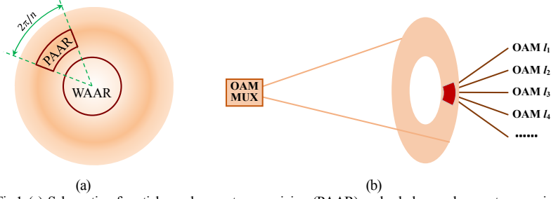
Fig.1 (a) Schematic of partial angular aperture receiving (PAAR) and whole angular aperture receiving (WAAR). (b) PAAR based OAM multiplexing communication system.
