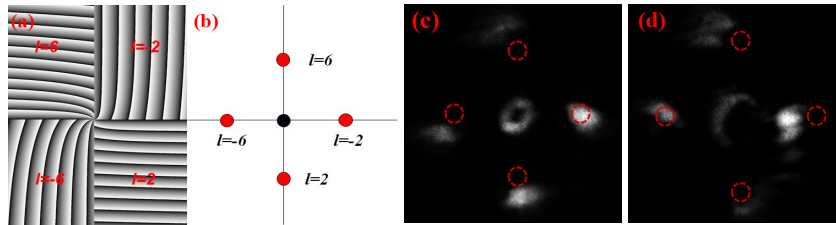
Fig.5 (a) The pattern combined with four hologram patterns designed for demultiplexing of OAM modes of -6, -2, 2, and 6 , each with an angular aperture of \pi/2 ; (b) the diffraction position for OAM modes of -6, -2, 2, and 6 ; (c) and (d) the measured diffraction images for the transmitting OAM modes of l=-2 and l=-6 , respectively.
