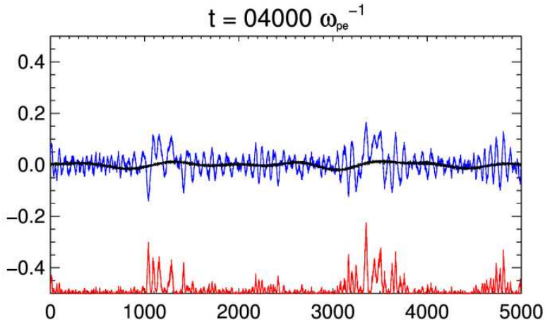
FIGURE 9. Embedded movie showing the wave packet evolution for \Delta n = 0.05 . The blue curve shows the spatial profile of the electric field E_x (V/m), the red shows 10E_X^2 - 0.5 , and the black shows the density profile \delta n/n_0 . Note to production staff: please embed movie "movie-fig9.avi" here
