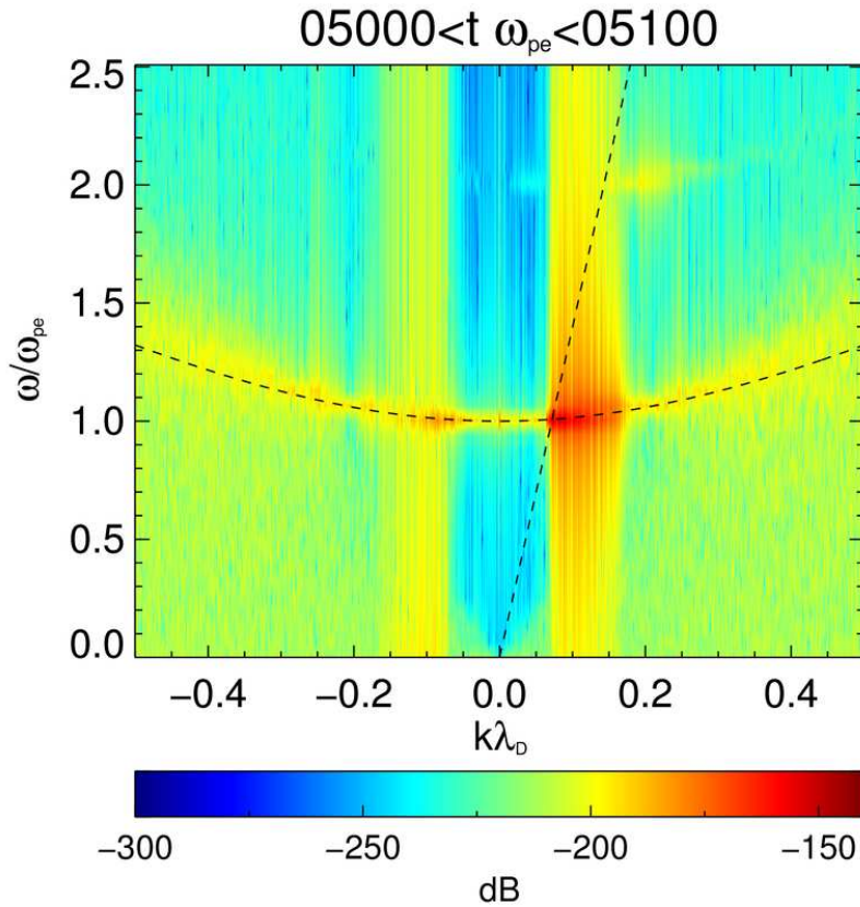
FIGURE 4. Embedded movie showing the evolution of time-windowed Fast Fourier Transforms of electric field energy in (k, \omega) -space for the homogeneous simulation. Note to production staff: please embed movie "movie-fig4.avi" here
