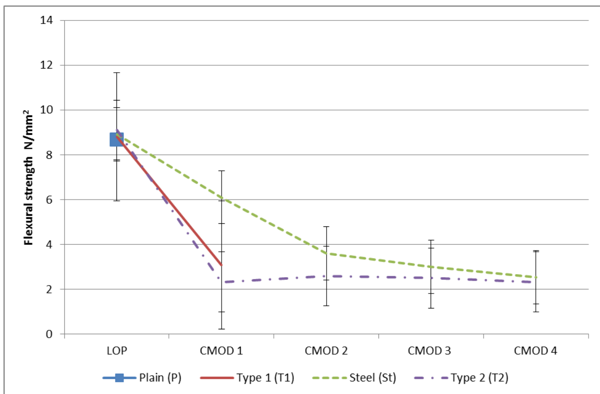
Figure 7 – Crack mouth opening displacement
