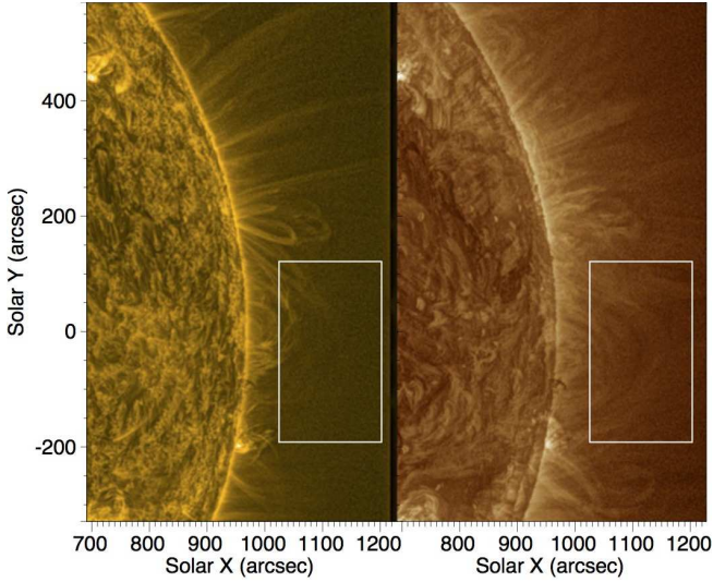
Figure 3. Similar to Figure 2 but showing the region QS4. The coronal structure is visible. The exact location for each set of footpoints is difficult to distinguish, with the coronal loops in 193 Å having higher/lower latitude footpoints (for northern/southern hemisphere footpoints) to the loops visible in 171 Å.
