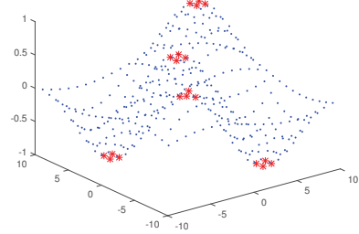
Fig. 12. The sub-regions with curvature values greater than 0.09
