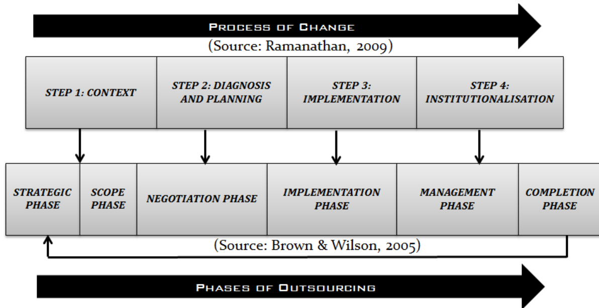
Figure 2: Conceptual Model
