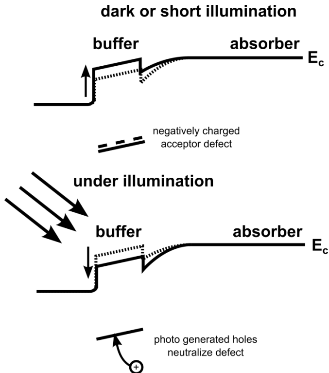
Figure 7. Schematic of the conduction band alignment in the presence of acceptor like deep defect states. In dark these defects are negatively charged due to trapping of electrons contributed from the donors of the buffer layer. This negative space charge decreases the band bending and increases the spike in the conduction band. Under illumination photogenerated holes can neutralize the defects resulting in a decrease of the spike.
