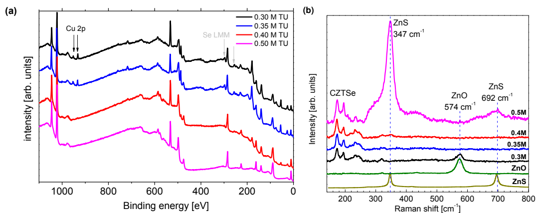
Figure 8. X-ray photoelectron spectroscopy (a) and UV-Raman (b) spectra and of ZnS(O,OH) buffer layer on CZTSe absorber deposited with different thiourea (TU) concentrations during the CBD process; ZnO and ZnS reference spectra were add for convenience.
