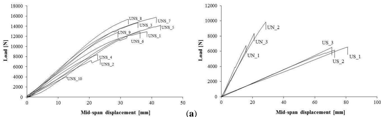
13 14 (b) 15 Figure 6. Load-Displacement curves: (a) control un-damaged beams; 16 (b) cut in half and notched beams.
