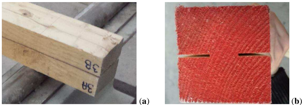
6 Figure 7. (a) Timber beams cut in half; (b) Notched beams.
