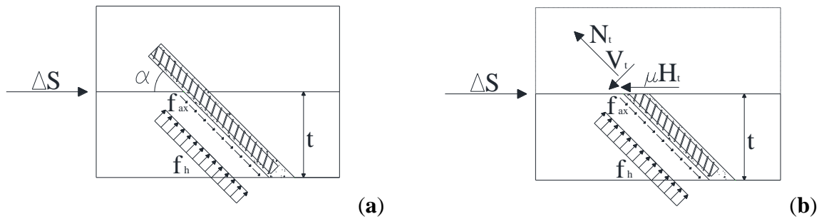
3 4 5 Figure 3. Failure mode A: (a) stresses in the joint; (b) load on the interface between the 6 timber elements.
