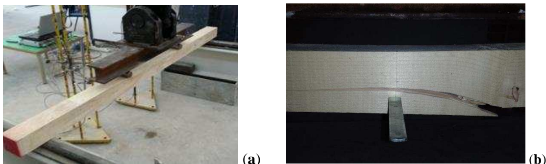
4 5 Figure 5. (a) Four-point-bending test setup; (b) Typical tensile failure mode of control 6 beams near a knot or due to grain deviation.
