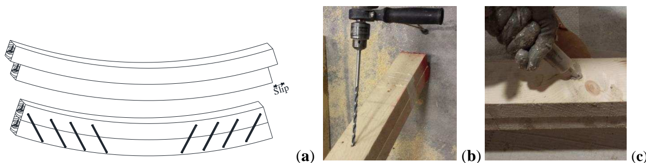
24 Figure 1. (a) Schematic arrangement of BFRP spikes; (b) Diagonal hole drilling, (c) Injection of epoxy putty.
