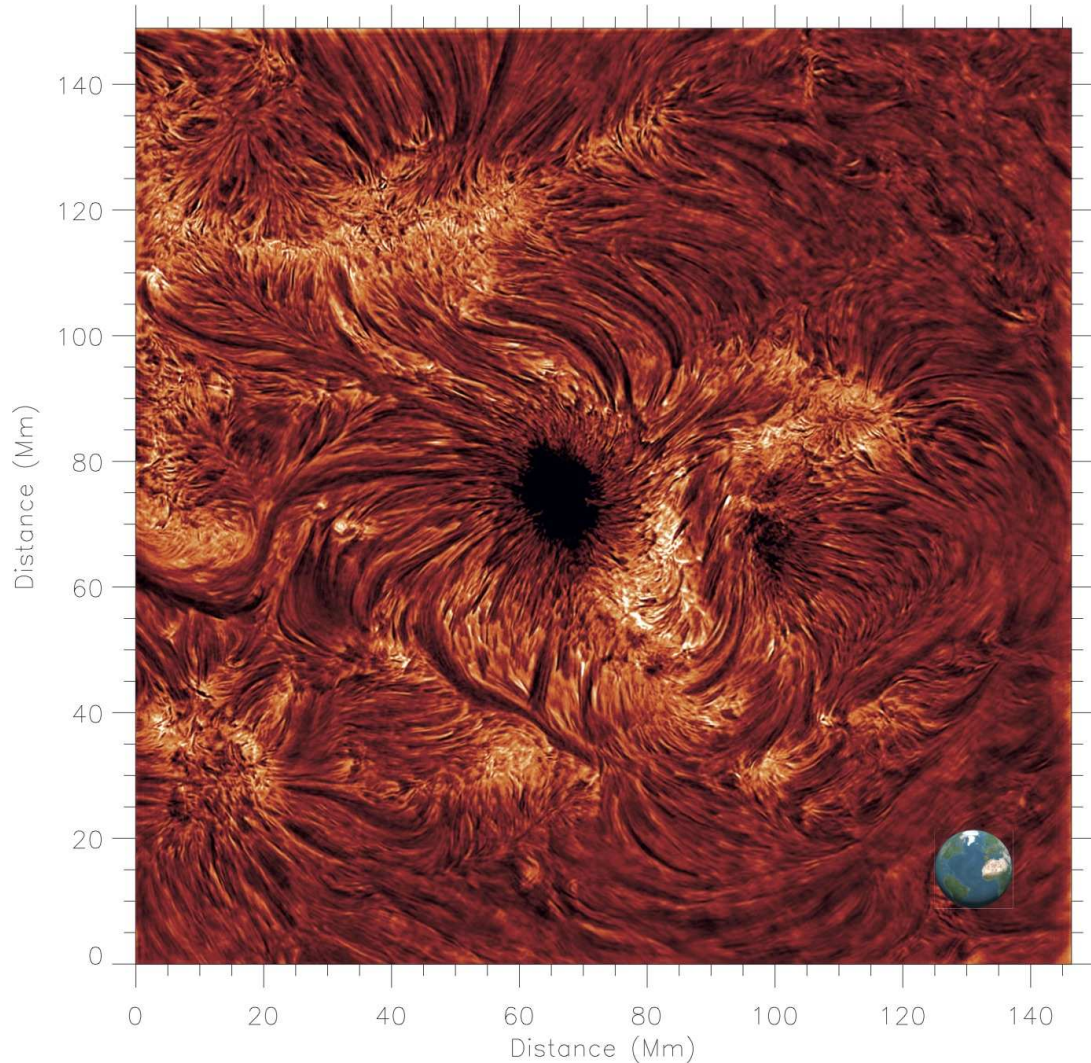
Fig. 2 An image of a solar active region acquired through a narrowband 0.25 \text{ \AA} H\alpha -core filter. Employing a new generation of large format, low noise CMOS sensors, it is now possible to obtain chromospheric fields-of-view in excess of 200'' \times 200'' (at the diffraction limit) with frame rates exceeding 60 \text{ s}^{-1} . A scale representation of the Earth is depicted in the lower-right section of the image. This snapshot, courtesy of D. B. Jess, was acquired using an Andor Technology 4.2 MP Zyla CMOS detector (15 ms exposure time at a frame rate of 64 \text{ s}^{-1} ) at the Dunn Solar Telescope, NM, USA.
