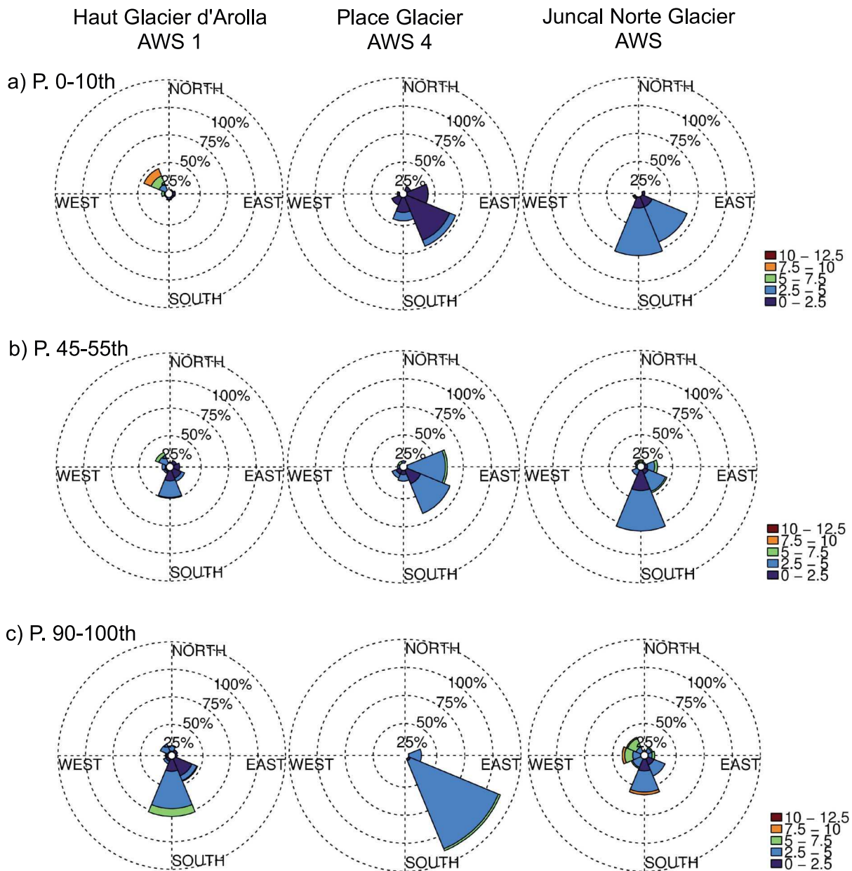
Figure 5. Wind roses at three representative AWS in respective glaciers. Wind distribution is shown for three percentiles ranges of the T_0 values. Wind speed in the legend is shown in m/s.
