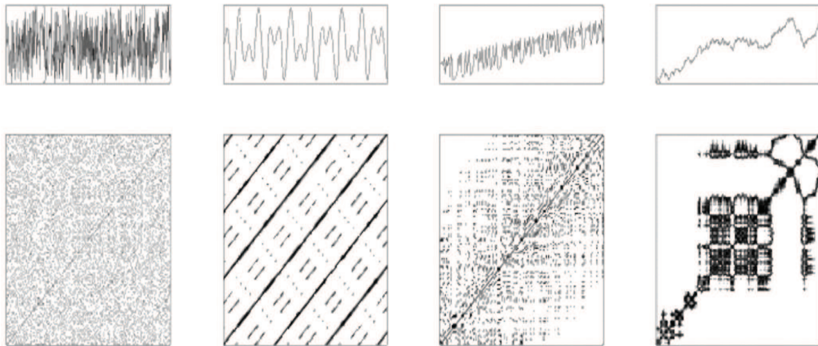
Figure 2. Illustration of the steps in RQA analysis.
