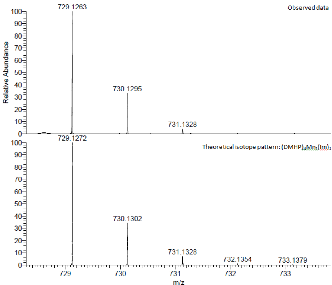
Figure 8: Detected m/z peak for [(DMPO)_4Mn_2(Im)_1]^+ (top) and its theoretical isotope pattern (bottom).
