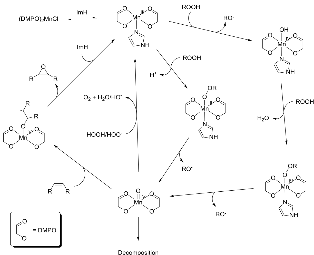
Scheme 8: Proposed mechanism for the epoxidation of alkenes.
