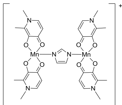
Scheme 4: Proposed structure for (DMPO)_4Mn_2(Im)_1 .
