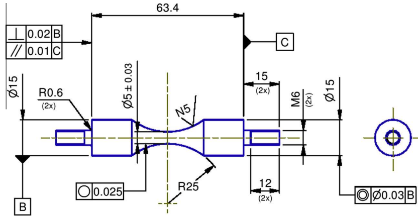
Fig. 2. Drawing of the HCF specimen.
