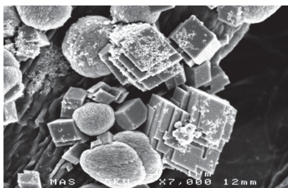
Figure 2. FE-SEM images of the cellulose mesh with calcite. The sample was previously coated with chromium to avoid charging in the SEM chamber.
