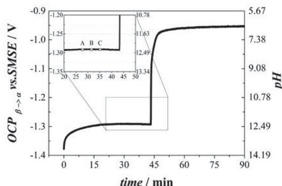
Figure 1. Potential transient (left axis) and corresponding pH (right axis) recorded with a 250 \mu\text{m} diameter nano-structured PdH microelectrode during the carbonation of a saturated \text{Ca}(\text{OH})_2 solution at 23^\circ\text{C} and 0.167 \text{atm } p_{\text{CO}_2} .
