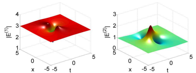
FIG. 1 (color online). Rogue waves envelope distributions |E^{(1)}(x, t)| and |E^{(2)}(x, t)| of Eq. (2). Here, a_1 = 3, a_2 = 1, q = 1, k = 2.36954 + 1.1972i and \lambda = -1.69162 - 1.79721i .
