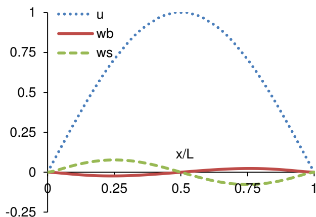
c. Third mode shape \omega_3 = 19.9412
