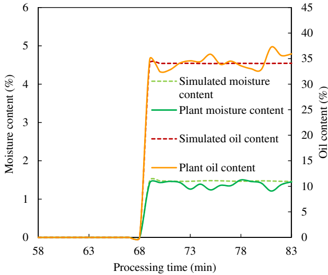
Fig. 9. Comparison of actual and predicted crisps moisture and oil content.
